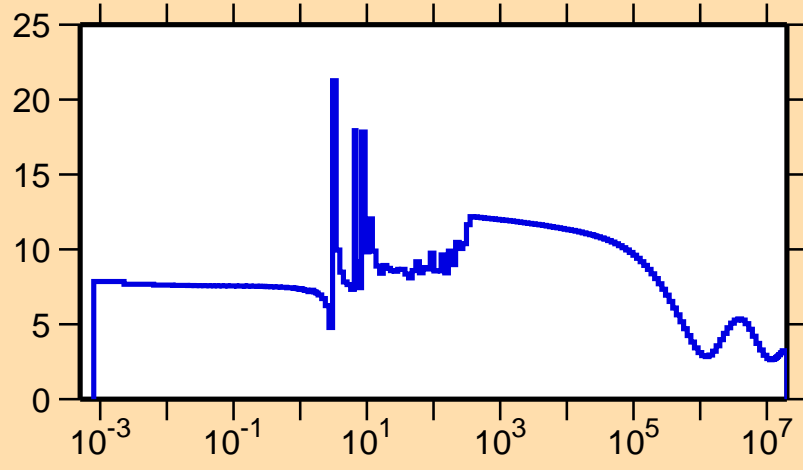
\sigma vs. E for ^{231}\text{Ac}(n,\text{el.})
