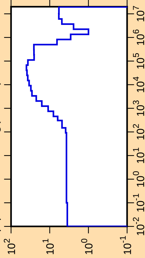
\Delta\mu/\mu vs. E for ^{101}\text{Ag}(\text{mt251})
