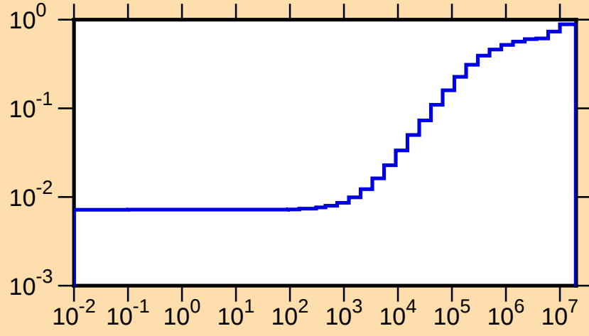
\mu vs. E for ^{101}\text{Ag}(\text{mt251})
