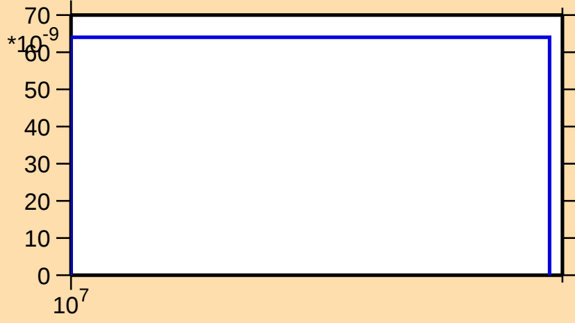
\sigma vs. E for ^{102}\text{Ag}(n,\text{pd})
