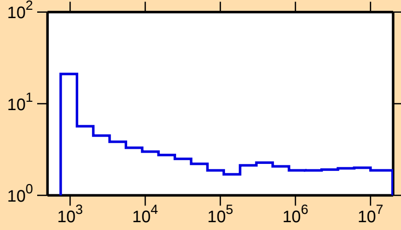
\sigma vs. E for ^{102}\text{Ag}(n,\text{nonel.})
