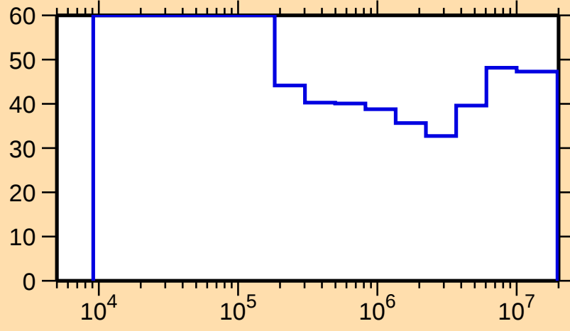
\Delta\sigma/\sigma vs. E for ^{102}\text{Ag}(n,n_1)
