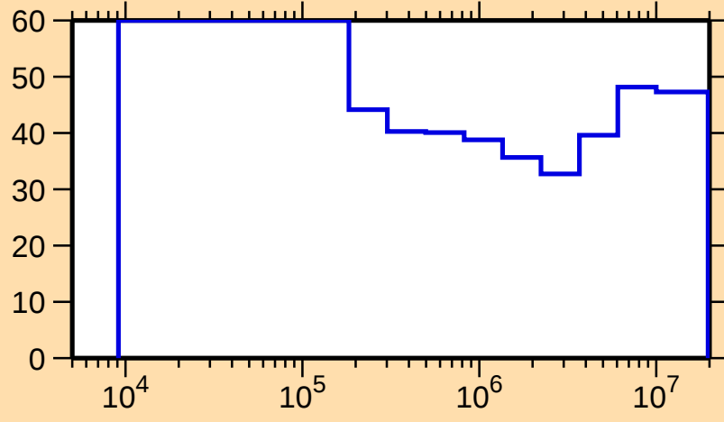
\Delta\sigma/\sigma vs. E for ^{102}\text{Ag}(n,n_1)
