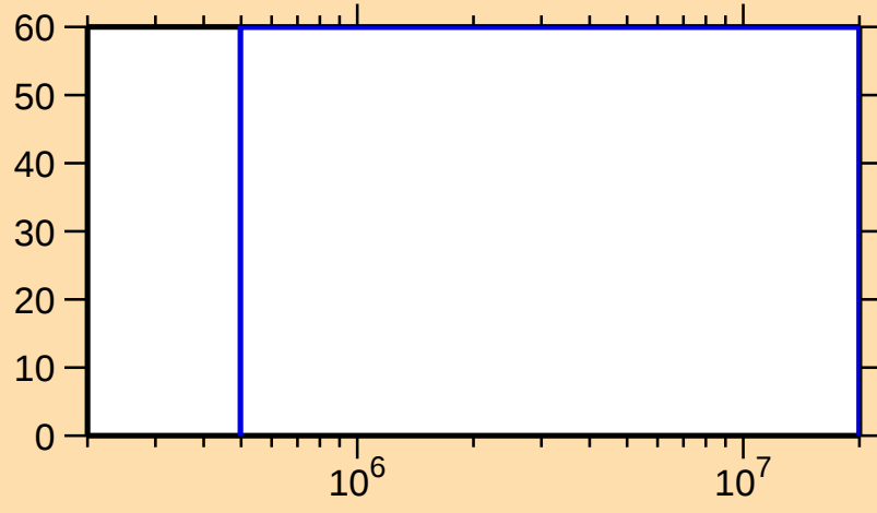
\Delta\sigma/\sigma vs. E for ^{118}\text{Ba}(n,n\text{cont.})
