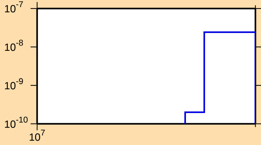
\sigma vs. E for ^{118}\text{Ba}(n,2n\alpha)
