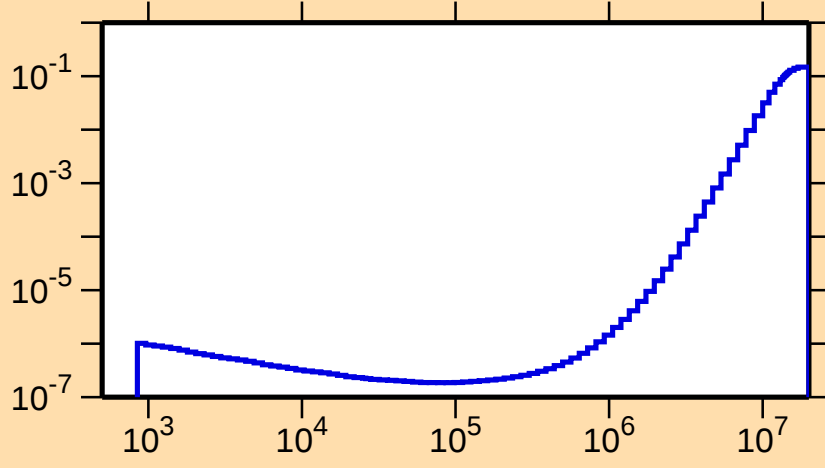
\sigma vs. E for ^{118}\text{Ba}(n,p\alpha)
