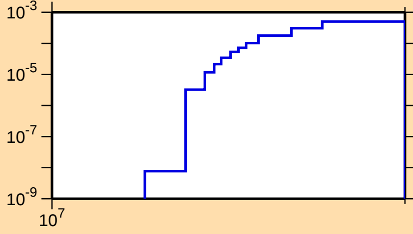
\sigma vs. E for ^{118}\text{Ba}(n,2n)
