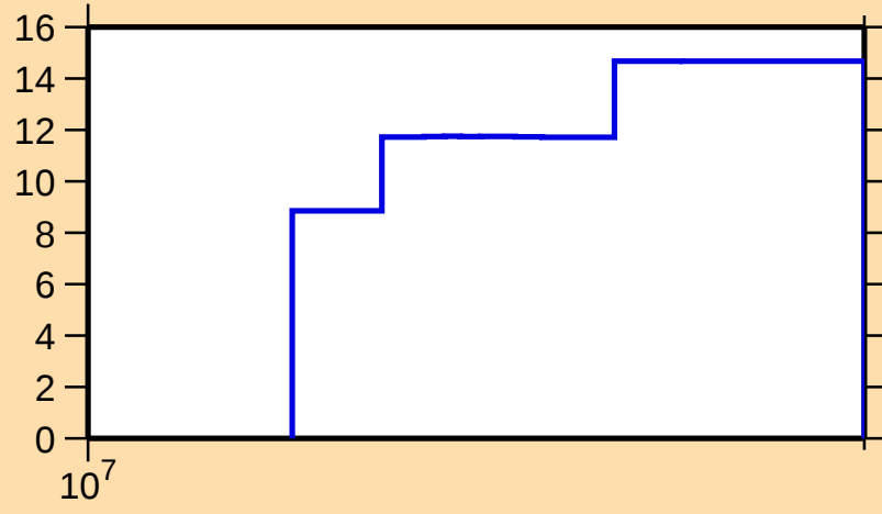
\Delta\sigma/\sigma vs. E for ^{118}\text{Ba}(n,\text{tot.})
