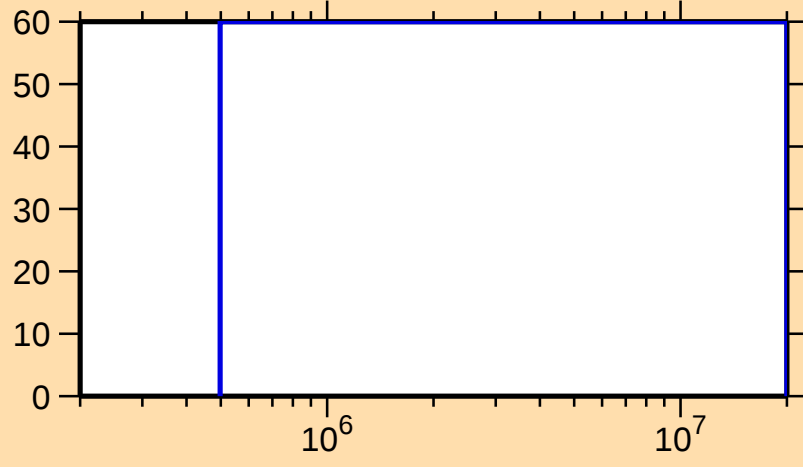
\Delta\sigma/\sigma vs. E for ^{118}\text{Ba}(n,n_1)
