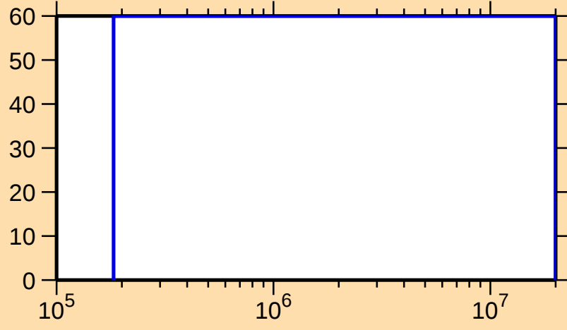
\Delta\sigma/\sigma vs. E for ^{118}\text{Ba}(n,\text{inel.})
