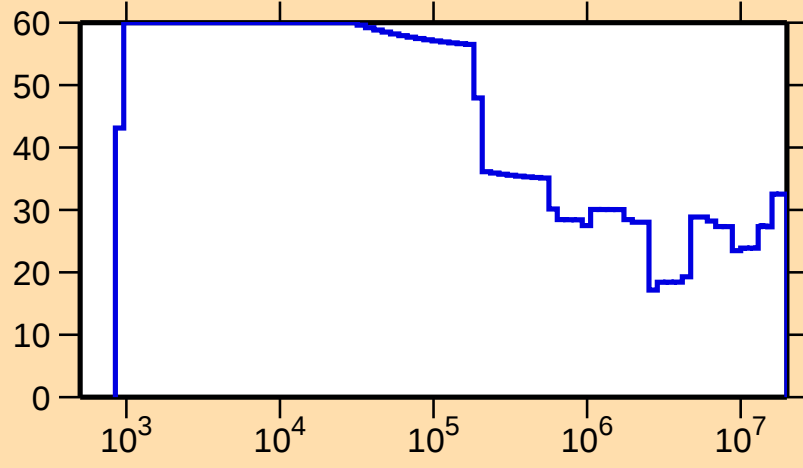
\Delta\sigma/\sigma vs. E for ^{118}\text{Ba}(n,\text{el.})
