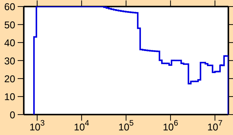
\Delta\sigma/\sigma vs. E for ^{118}\text{Ba}(n,\text{el.})
