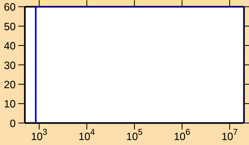
\Delta\sigma/\sigma vs. E for ^{118}\text{Ba}(n,\gamma)
