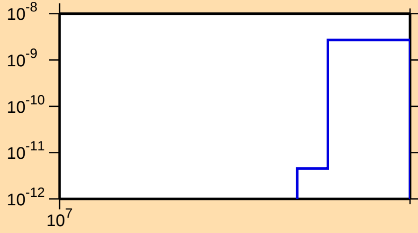
\sigma vs. E for ^{118}\text{Ba}(n,\text{nd})
