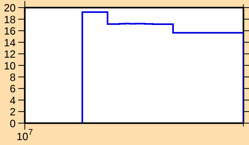
\Delta\sigma/\sigma vs. E for ^{118}\text{Ba}(n,\text{nonel.})
