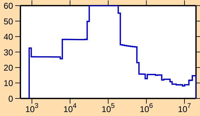
\Delta\sigma/\sigma vs. E for ^{118}\text{Ba}(n,\text{tot.})
