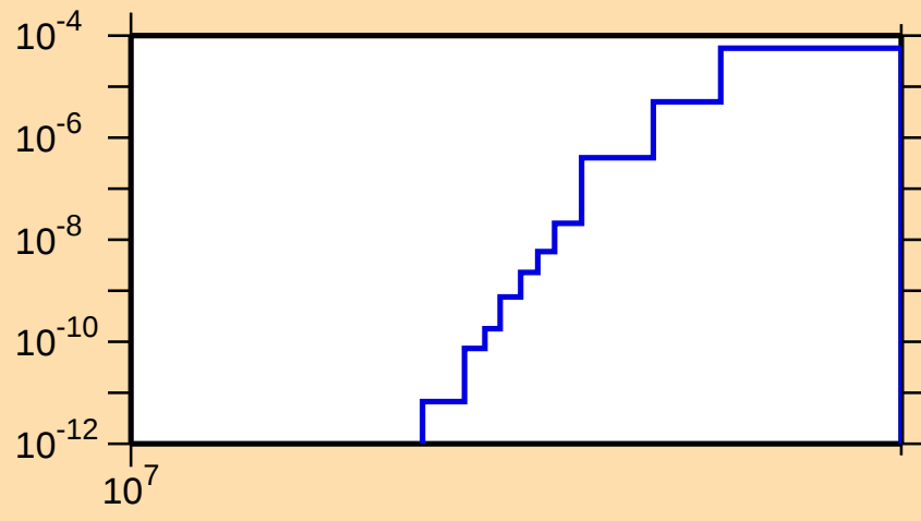
\sigma vs. E for ^{118}\text{Ba}(n,\text{pt})
