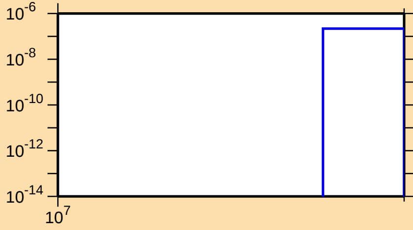
\sigma vs. E for ^{118}\text{Ba}(n,2np)
