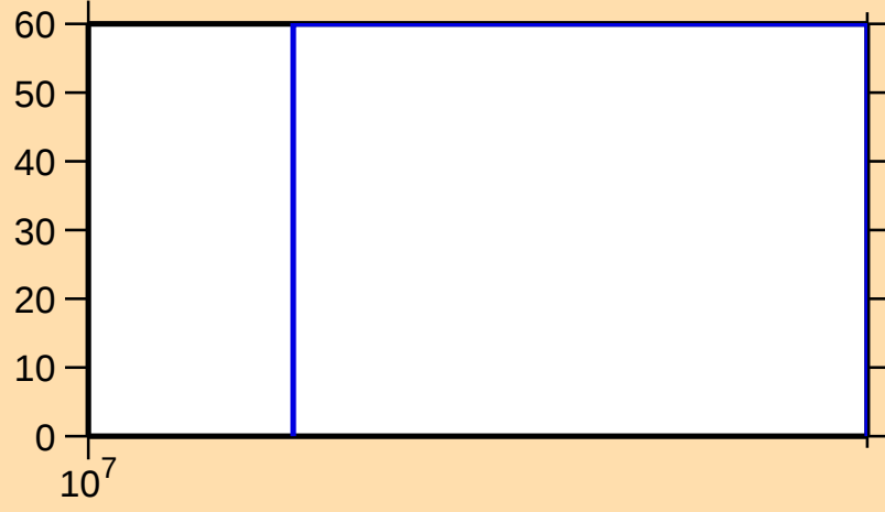
\Delta\sigma/\sigma vs. E for ^{118}\text{Ba}(n,\text{inel.})
