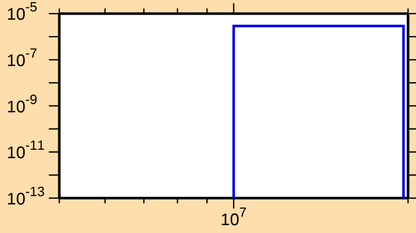
\sigma vs. E for ^{138}\text{Ba}(n,t)
