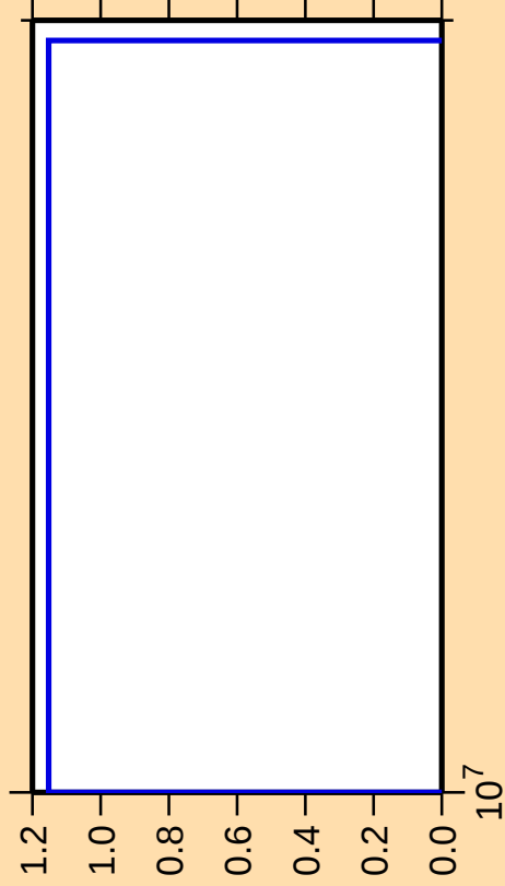
\Delta\sigma/\sigma vs. E for ^{138}\text{Ba}(n,\text{nt})
