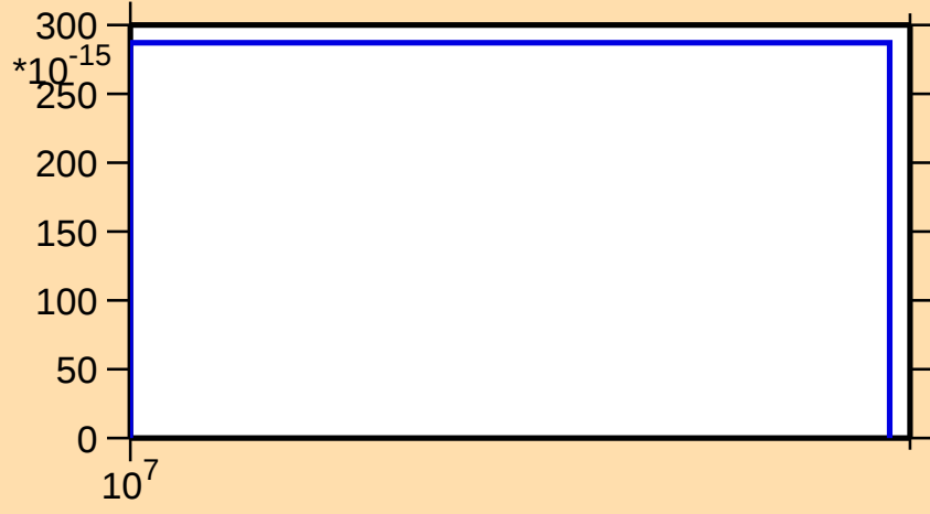
\sigma vs. E for ^{138}\text{Ba}(n,\text{nt})
