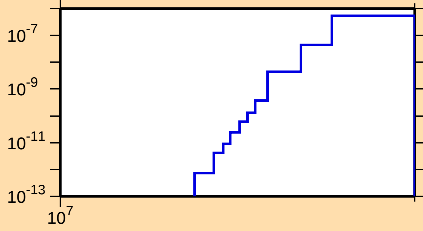
\sigma vs. E for ^{241}\text{Bk}(n,\text{nd})
