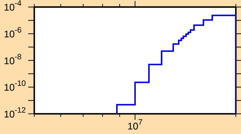
\sigma vs. E for ^{241}\text{Bk}(\text{mt117})
