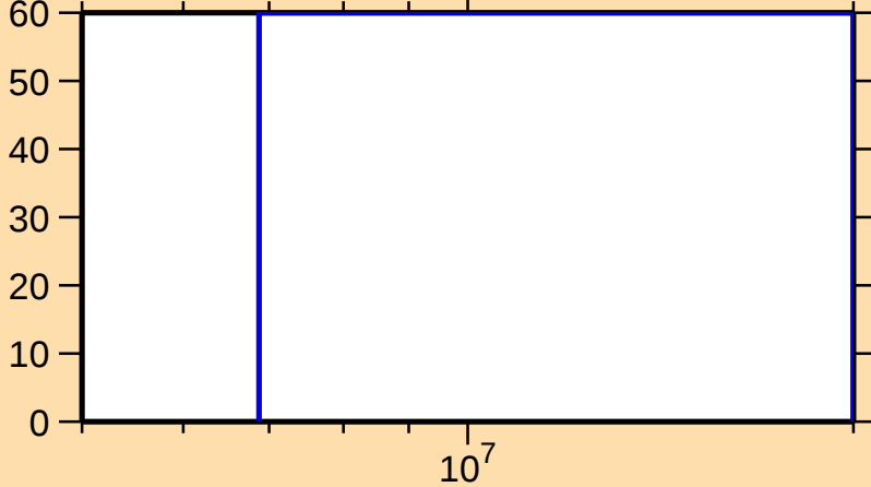
\Delta\sigma/\sigma vs. E for ^{241}\text{Bk}(n,2n)
