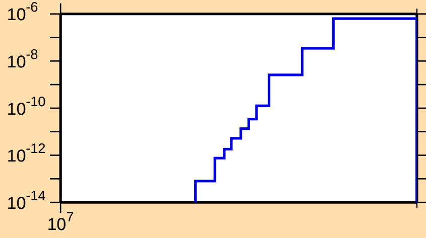
\sigma vs. E for ^{241}\text{Bk}(n,nt)
