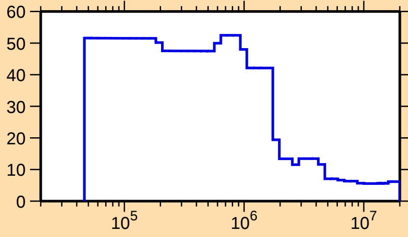
\Delta\sigma/\sigma vs. E for ^{241}\text{Bk}(n,\text{nonel.})
