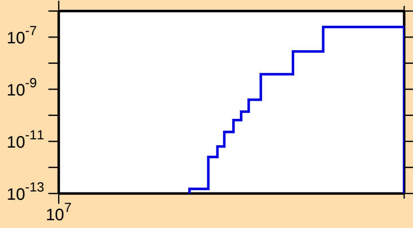
\sigma vs. E for ^{241}\text{Bk}(n,2np)
