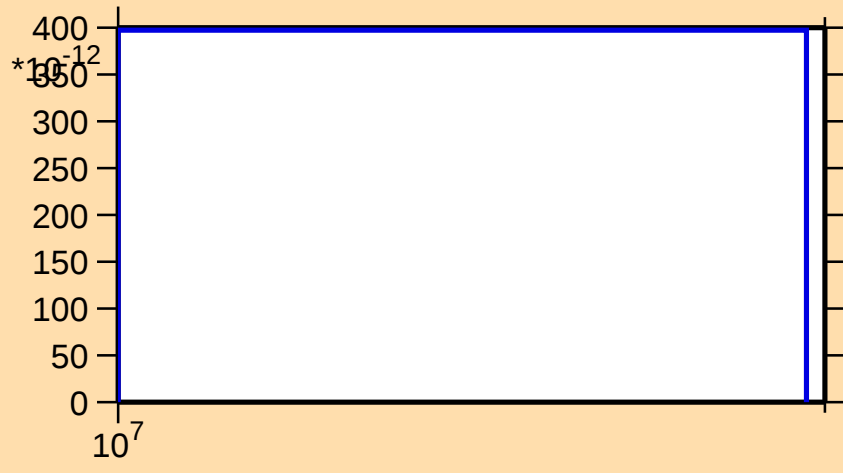
\sigma vs. E for ^{241}\text{Bk}(n,\text{He3})
