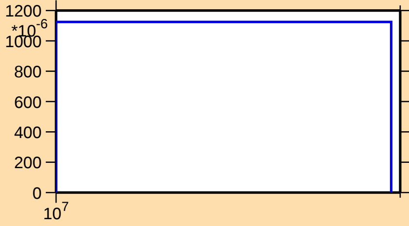
\sigma vs. E for ^{241}\text{Bk}(n,3n)
