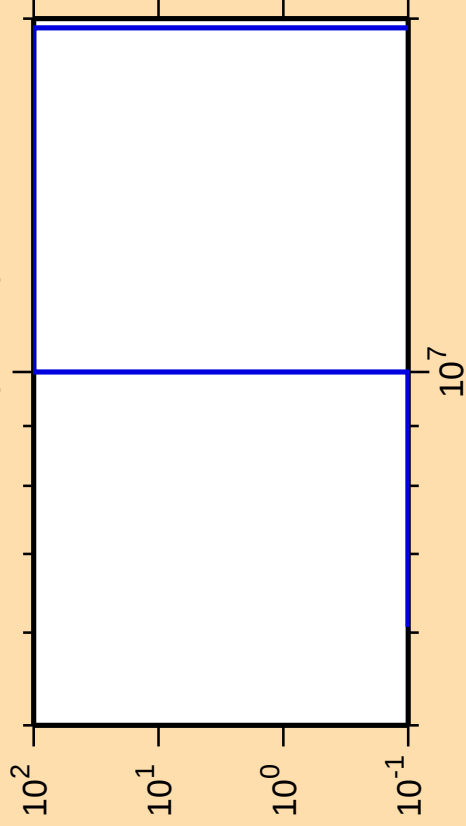
\Delta\sigma/\sigma vs. E for ^{241}\text{Bk}(\text{mt } 45)
