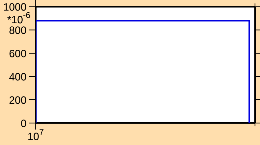
\sigma vs. E for ^{241}\text{Bk}(n,3n\alpha)
