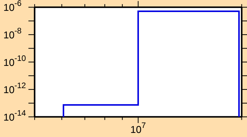
\sigma vs. E for ^{241}\text{Bk}(\text{mt } 45)
