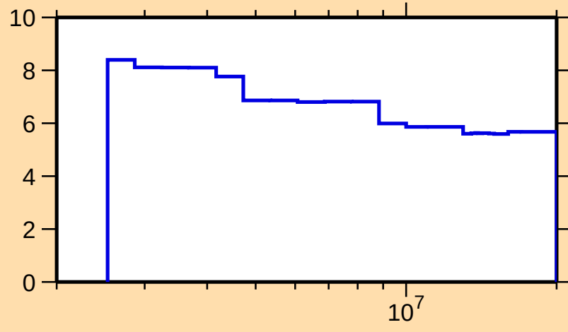
\Delta\sigma/\sigma vs. E for ^{83}\text{Br}(n,n\text{oncl.})
