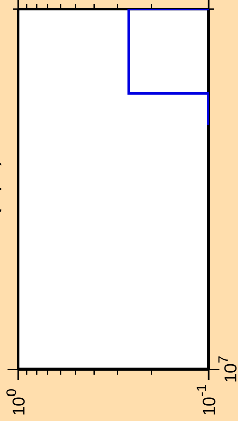
\Delta\sigma/\sigma vs. E for ^{83}\text{Br}(n,p\alpha)
