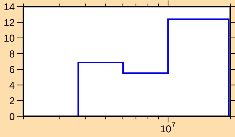
\Delta\sigma/\sigma vs. E for ^{83}\text{Br}(n,\text{el.})
