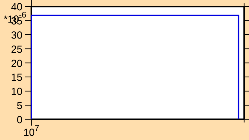
\sigma vs. E for ^{83}\text{Br}(n,3n)
