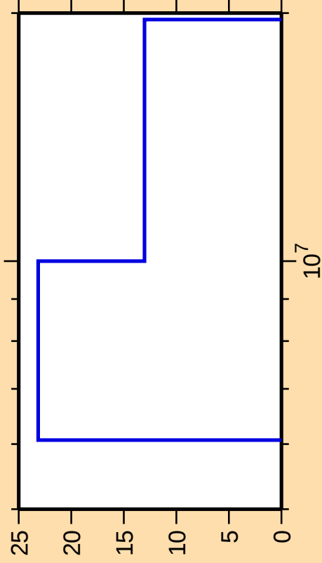
\Delta\sigma/\sigma vs. E for ^{83}\text{Br}(n,2n)
