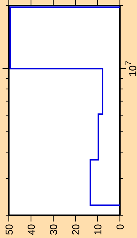
\Delta\sigma/\sigma vs. E for ^{83}\text{Br}(\text{n},\text{ncont.})
