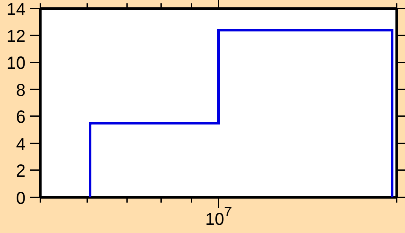
\Delta\sigma/\sigma vs. E for ^{83}\text{Br}(n,\text{el.})
