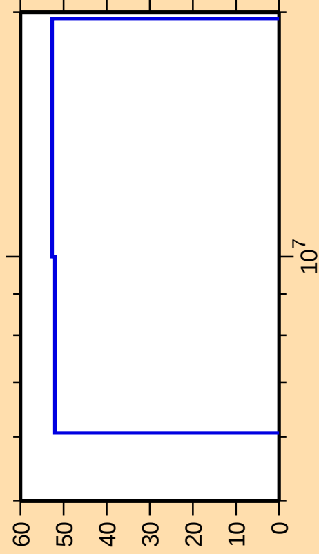
\Delta\sigma/\sigma vs. E for ^{83}\text{Br}(n,d)
