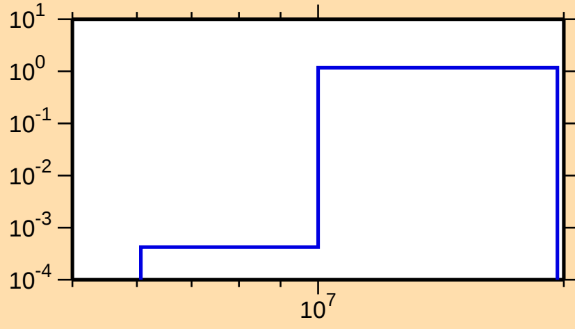
\sigma vs. E for ^{83}\text{Br}(n,2n)
