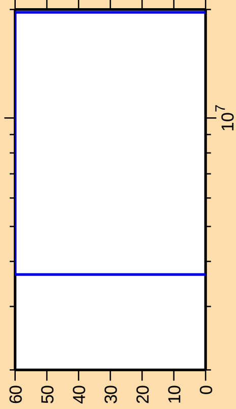
\Delta\sigma/\sigma vs. E for ^{83}\text{Br}(n,\alpha)
