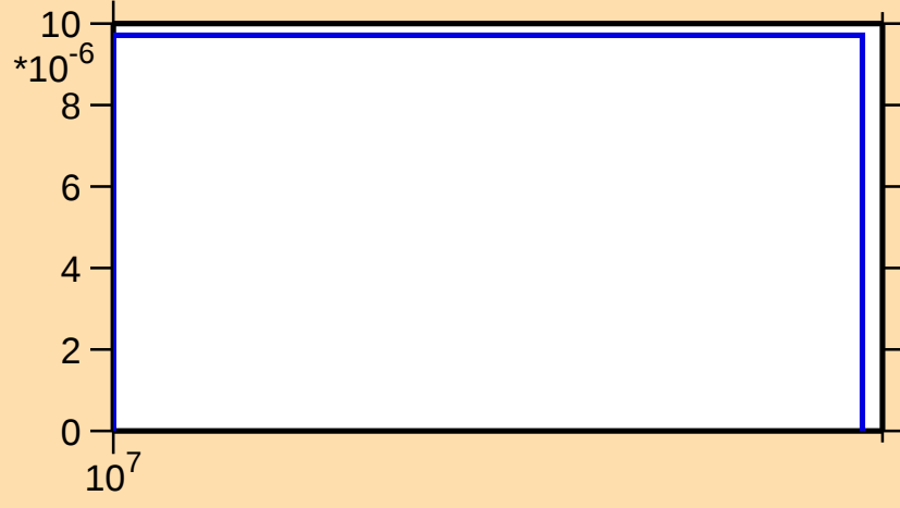
\sigma vs. E for ^{83}\text{Br}(n,n\alpha)
