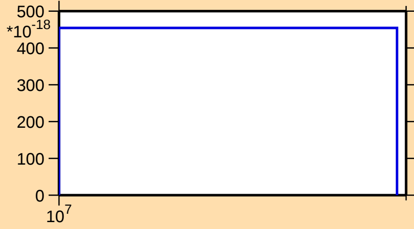
\sigma vs. E for ^{83}\text{Br}(n,p\alpha)
