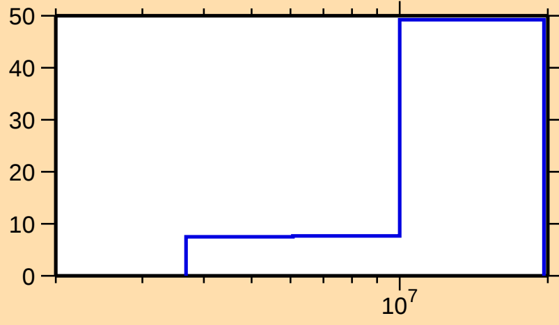
\Delta\sigma/\sigma vs. E for ^{83}\text{Br}(n,\text{inel.})
