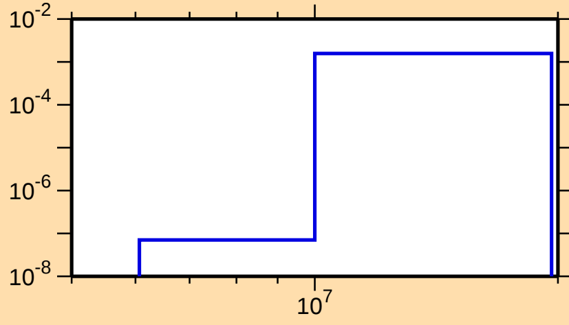
\sigma vs. E for ^{83}\text{Br}(n,d)
