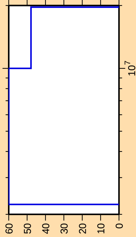
\Delta\sigma/\sigma vs. E for ^{83}\text{Br}(n,\gamma)
