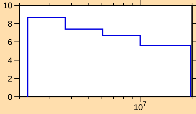
\Delta\sigma/\sigma vs. E for ^{83}\text{Br}(\text{n},\text{nonel.})
