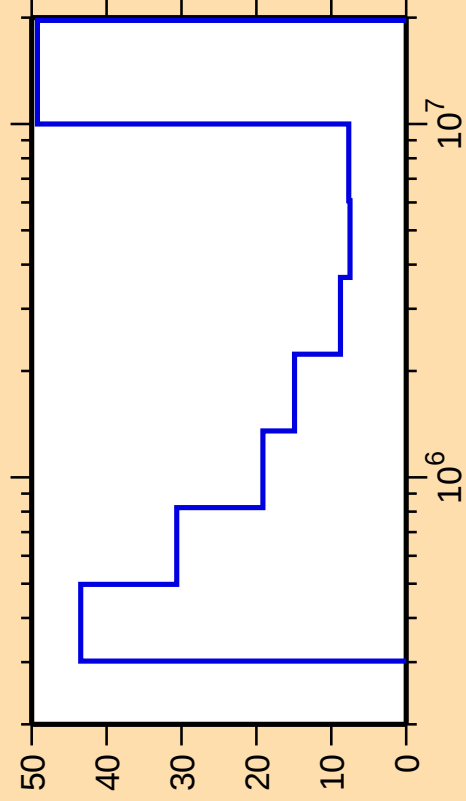
\Delta\sigma/\sigma vs. E for ^{83}\text{Br}(n,\text{inel.})
