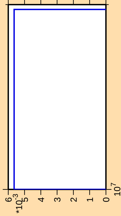
\Delta\sigma/\sigma vs. E for ^{83}\text{Br}(n,\text{He3})
