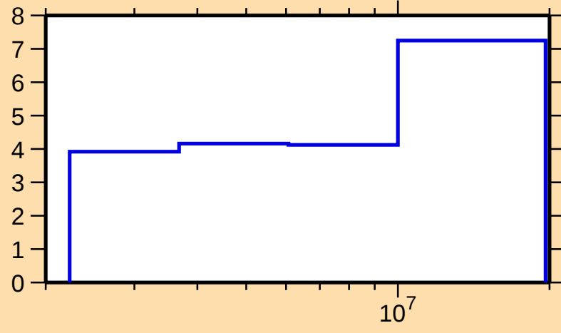
\Delta\sigma/\sigma vs. E for ^{83}\text{Br}(n,\text{tot.})
