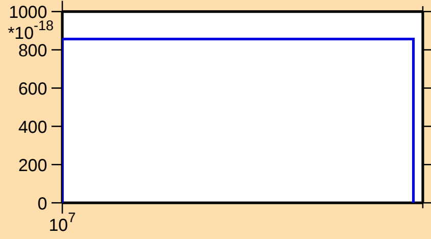
\sigma vs. E for ^{83}\text{Br}(n,\text{He3})
