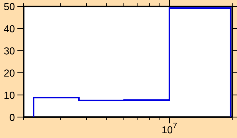
\Delta\sigma/\sigma vs. E for ^{83}\text{Br}(\text{n},\text{inel.})
