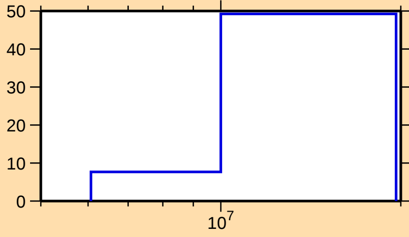
\Delta\sigma/\sigma vs. E for ^{83}\text{Br}(n,\text{inel.})
