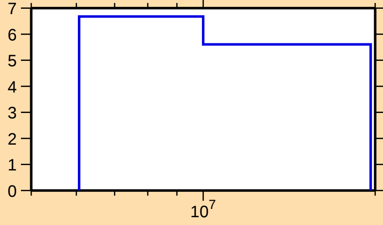
\Delta\sigma/\sigma vs. E for ^{83}\text{Br}(n,\text{nonel.})
