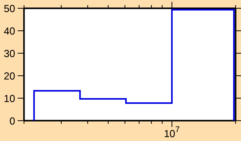
\Delta\sigma/\sigma vs. E for ^{83}\text{Br}(n,n\text{cont.})
