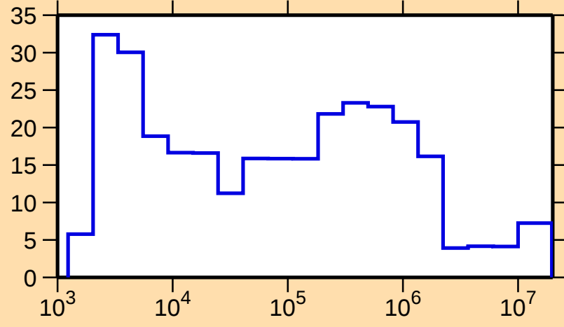
\Delta\sigma/\sigma vs. E for ^{83}\text{Br}(n,\text{tot.})
