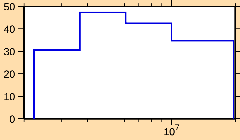
\Delta\sigma/\sigma vs. E for ^{83}\text{Br}(n, n_1)
