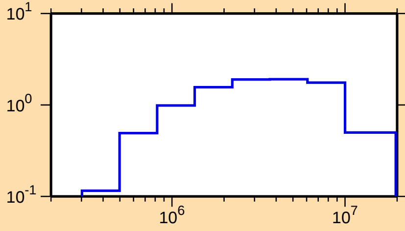
\sigma vs. E for ^{83}\text{Br}(n,\text{inel.})
