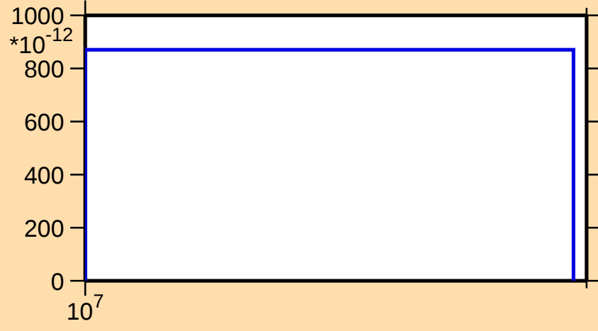
\sigma vs. E for ^{83}\text{Br}(n,\text{nd})
