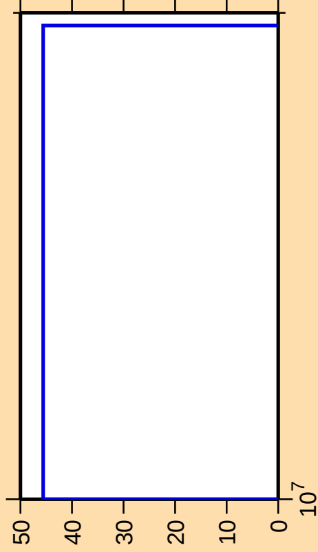
\Delta\sigma/\sigma vs. E for ^{83}\text{Br}(n,3n)
