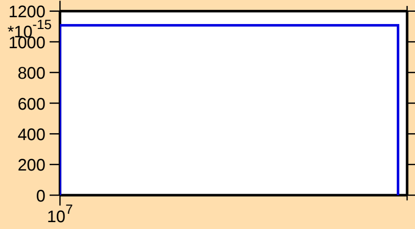
\sigma vs. E for ^{83}\text{Br}(n,2np)
