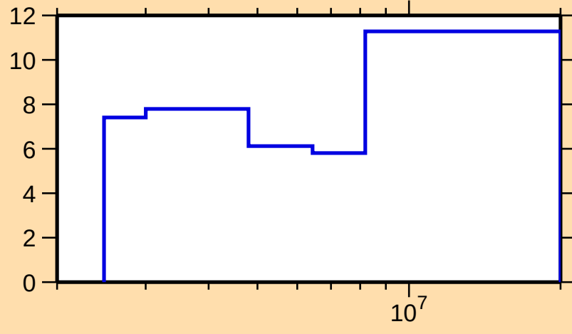
\Delta\sigma/\sigma vs. E for ^{83}\text{Br}(\text{n},\text{el.})
