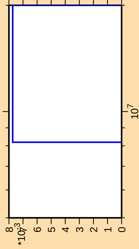
\Delta\sigma/\sigma vs. E for ^{83}\text{Br}(n,\text{He3})
