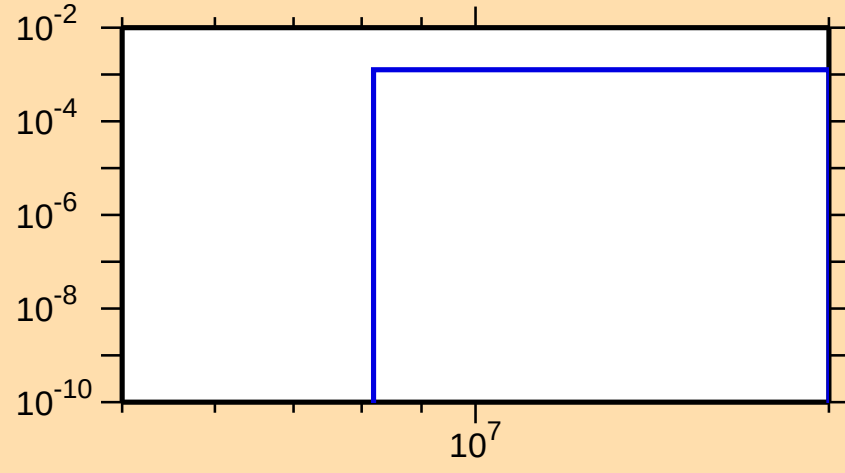
\sigma vs. E for ^{83}\text{Br}(n,d)
