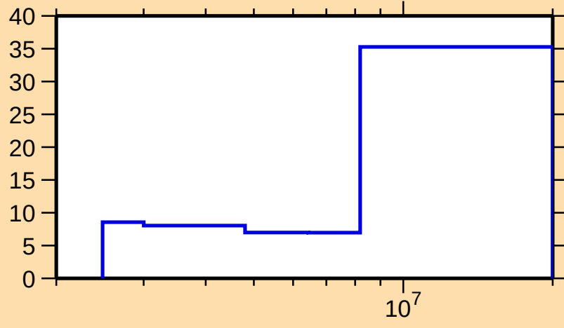
\Delta\sigma/\sigma vs. E for ^{83}\text{Br}(\text{n},\text{inel.})
