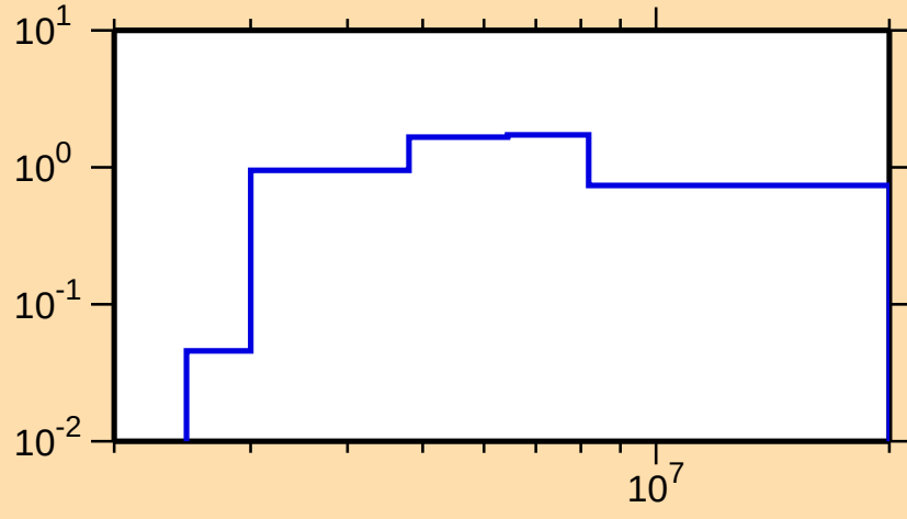
\sigma vs. E for ^{83}\text{Br}(n,n\text{cont.})
