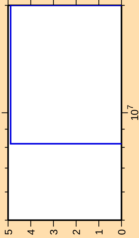
\Delta\sigma/\sigma vs. E for ^{83}\text{Br}(n,2np)
