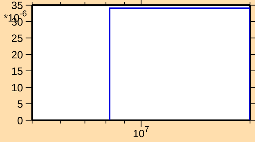
\sigma vs. E for ^{83}\text{Br}(n,3n)
