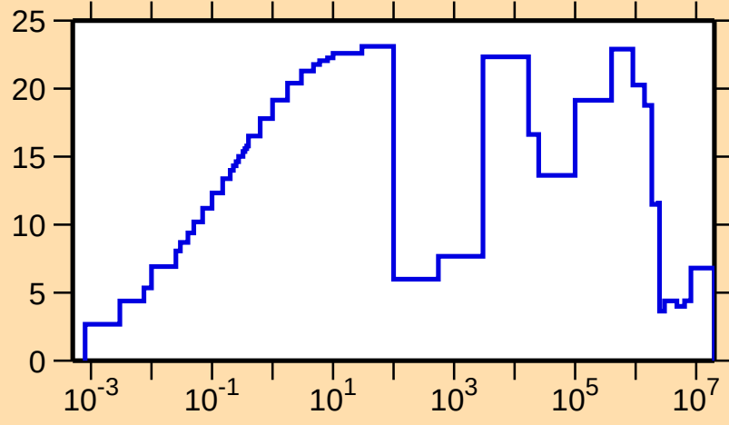
\Delta\sigma/\sigma vs. E for ^{83}\text{Br}(n,\text{tot.})
