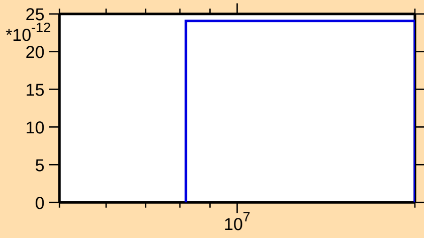
\sigma vs. E for ^{83}\text{Br}(n,\text{nt})
