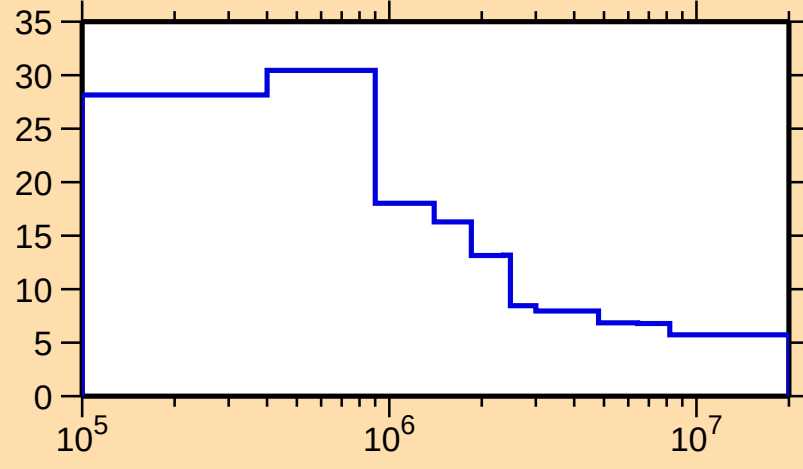
\Delta\sigma/\sigma vs. E for ^{83}\text{Br}(n,\text{nonel.})
