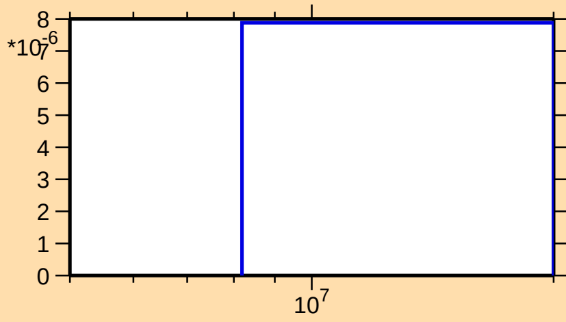
\sigma vs. E for ^{83}\text{Br}(n,\alpha)
