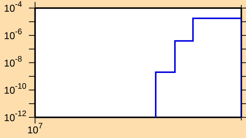
\sigma vs. E for ^{88}\text{Br}(n,nt)
