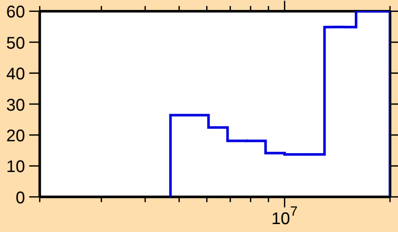
\Delta\sigma/\sigma vs. E for ^{88}\text{Br}(n,2n)
