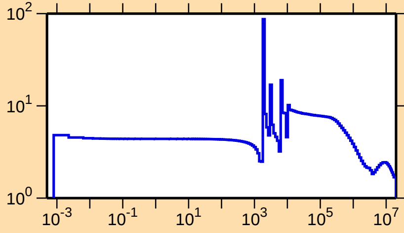
\sigma vs. E for ^{88}\text{Br}(n,\text{el.})
