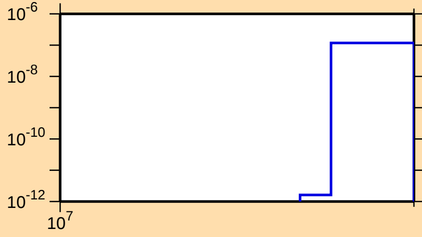
\sigma vs. E for ^{88}\text{Br}(n,2np)
