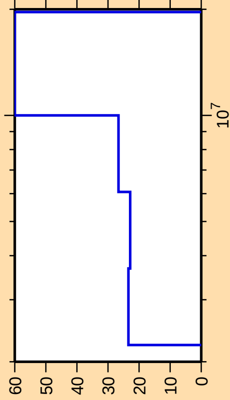
\Delta\sigma/\sigma vs. E for ^{88}\text{Br}(\text{n},\text{ncont.})
