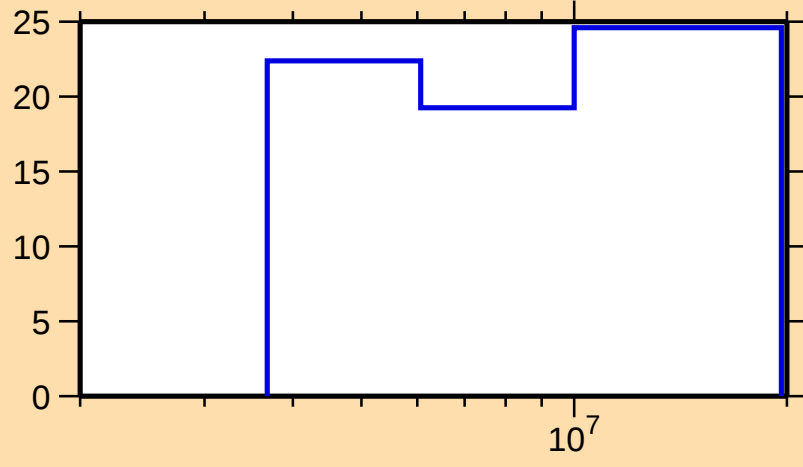
\Delta\sigma/\sigma vs. E for ^{88}\text{Br}(n,\text{el.})
