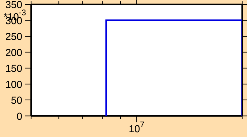
\sigma vs. E for ^{88}\text{Br}(n,3n)
