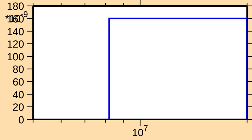
\sigma vs. E for ^{88}\text{Br}(n,\text{nt})
