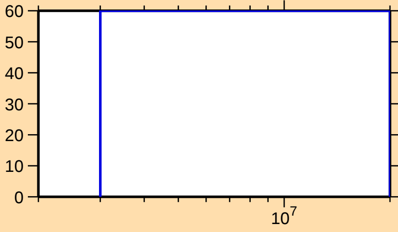
\Delta\sigma/\sigma vs. E for ^{88}\text{Br}(n,n_1)
