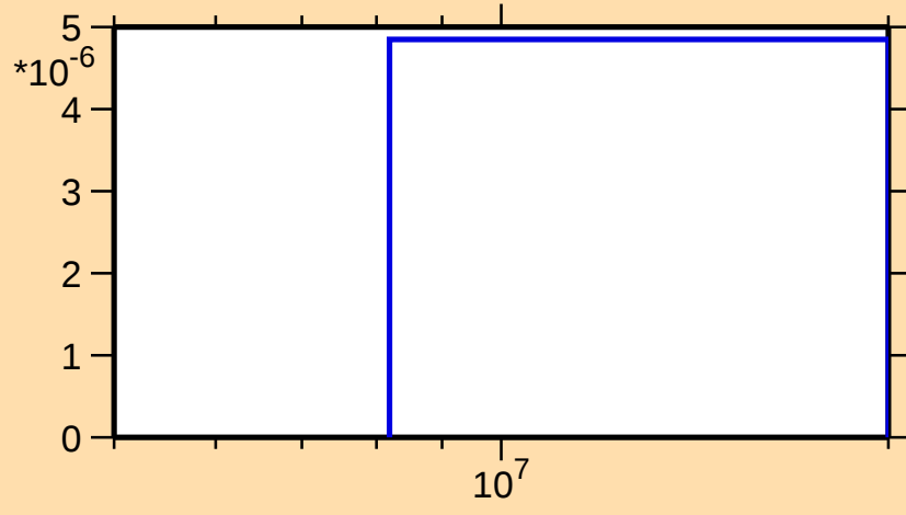
\sigma vs. E for ^{88}\text{Br}(n,\alpha)
