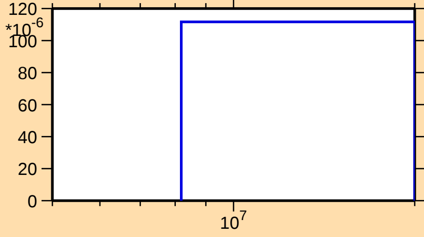
\sigma vs. E for ^{88}\text{Br}(n,d)
