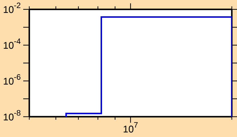
\sigma vs. E for ^{88}\text{Br}(n,p)
