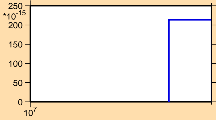
\sigma vs. E for ^{40}\text{Ca}(n,pt)
