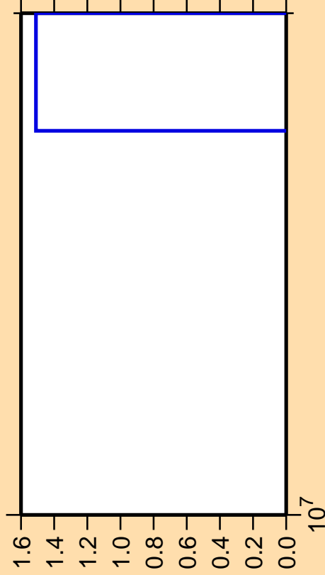
\Delta\sigma/\sigma vs. E for ^{40}\text{Ca}(n,pt)
