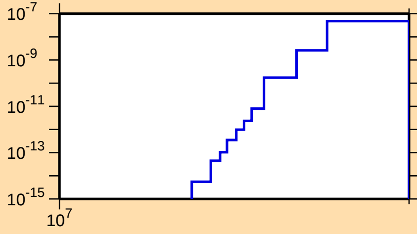
\sigma vs. E for ^{104}\text{Cd}(\text{mt117})
