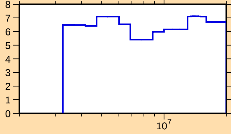
\Delta\sigma/\sigma vs. E for ^{104}\text{Cd}(n,n\text{onel.})
