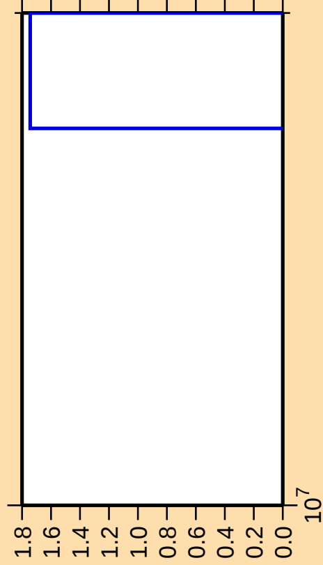
\Delta\sigma/\sigma vs. E for ^{104}\text{Cd}(n,nt)
