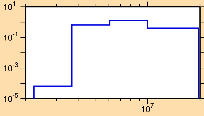
\sigma vs. E for ^{104}\text{Cd}(n,n\text{cont.})
