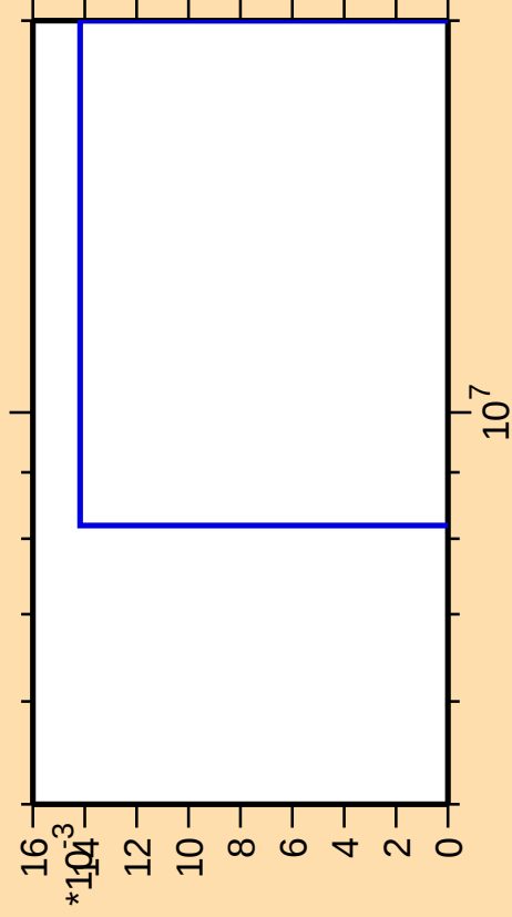
\Delta\sigma/\sigma vs. E for ^{104}\text{Cd}(n,nt)
