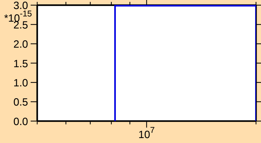
\sigma vs. E for ^{104}\text{Cd}(n,nt)
