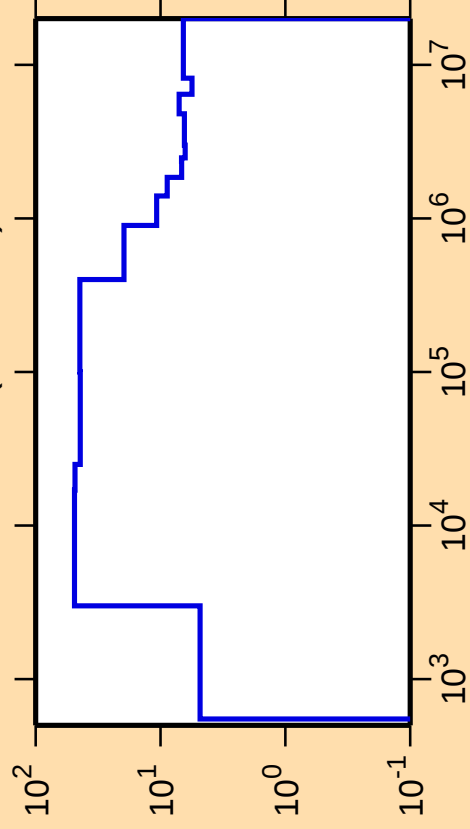
\Delta\sigma/\sigma vs. E for ^{104}\text{Cd}(n,\text{nonel.})
