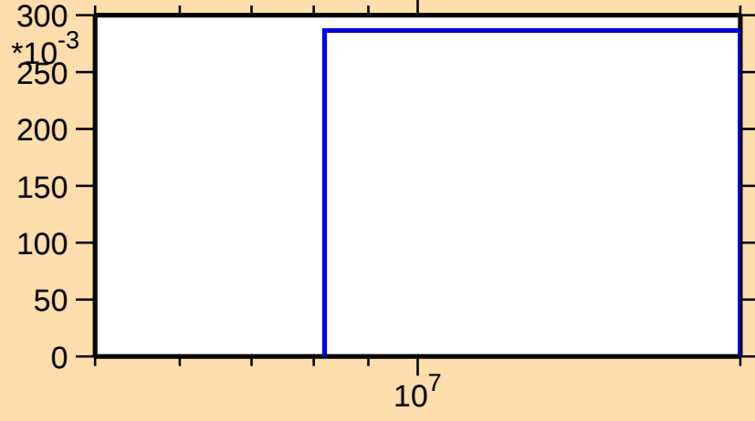
\sigma vs. E for ^{104}\text{Cd}(n,2n)
