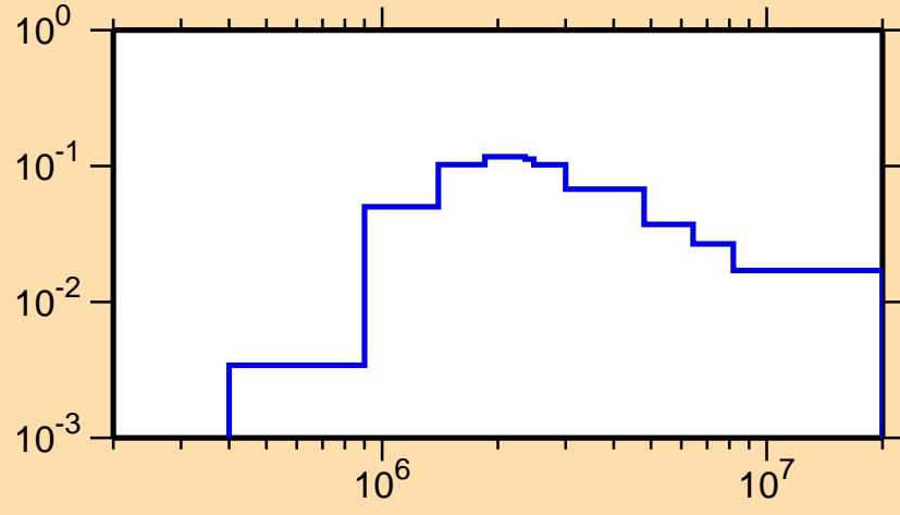
\sigma vs. E for ^{128}\text{Ce}(n,n_2)
