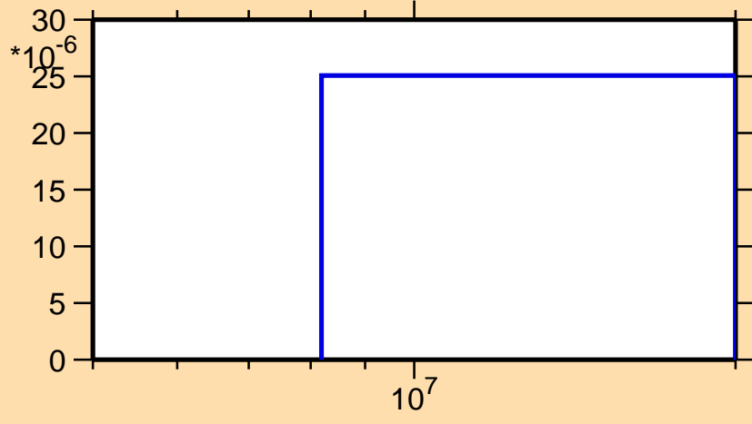
\sigma vs. E for ^{128}\text{Ce}(n,t)
