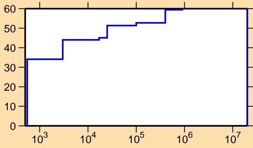
\Delta\sigma/\sigma vs. E for ^{128}\text{Ce}(n,\gamma)
