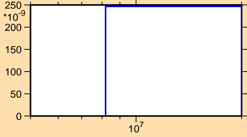
\sigma vs. E for ^{128}\text{Ce}(\text{mt } 45)
