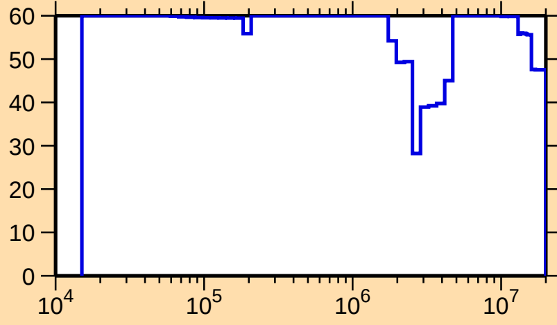
\Delta\sigma/\sigma vs. E for ^{122}\text{Cs}(n,n_1)
