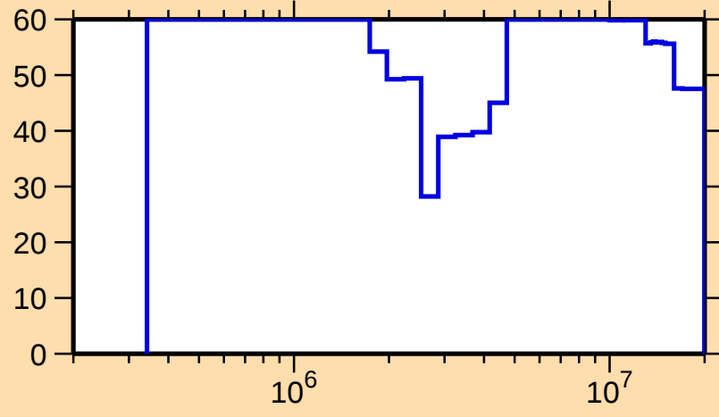
\Delta\sigma/\sigma vs. E for ^{122}\text{Cs}(n,n_1)
