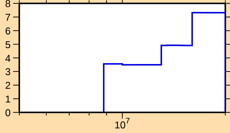
\Delta\sigma/\sigma vs. E for ^{122}\text{Cs}(n,\text{nonel.})
