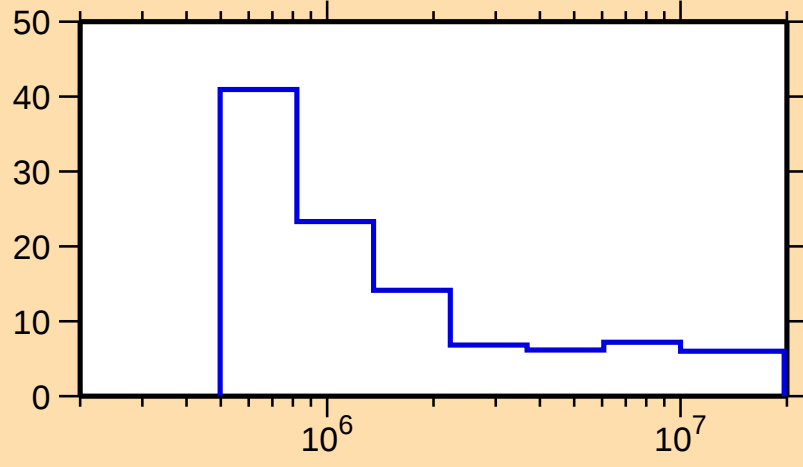
\Delta\sigma/\sigma vs. E for ^{139}\text{Cs}(n,\text{nonel.})
