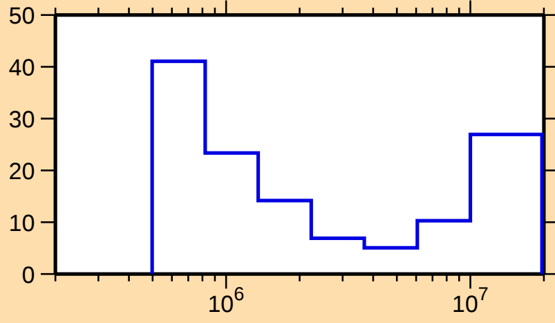
\Delta\sigma/\sigma vs. E for ^{139}\text{Cs}(n,\text{inel.})
