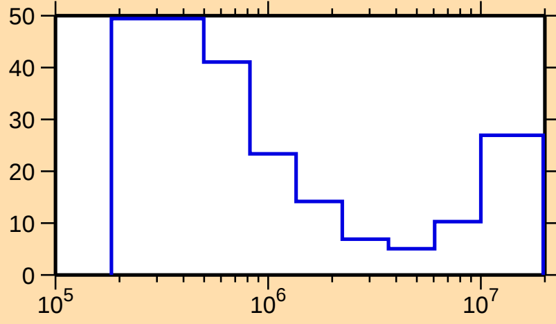
\Delta\sigma/\sigma vs. E for ^{139}\text{Cs}(n,\text{inel.})
