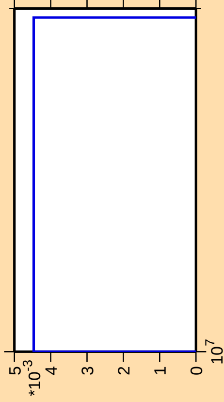
\Delta\sigma/\sigma vs. E for ^{139}\text{Cs}(n,3n\alpha)
