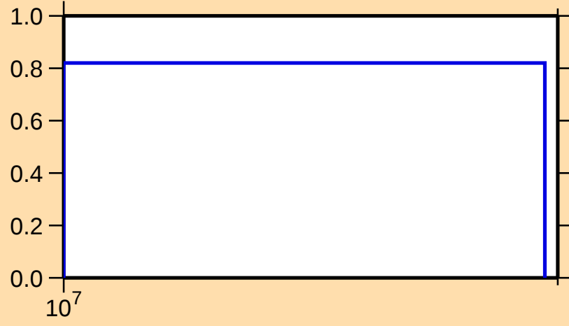
\sigma vs. E for ^{139}\text{Cs}(n,3n)
