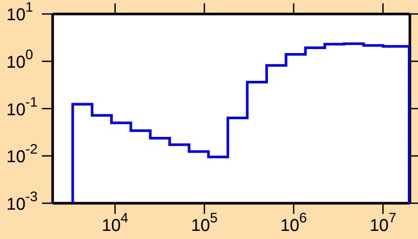
\sigma vs. E for ^{139}\text{Cs}(n,\text{nonel.})
