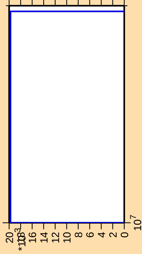
\Delta\sigma/\sigma vs. E for ^{139}\text{Cs} (mt 45)
