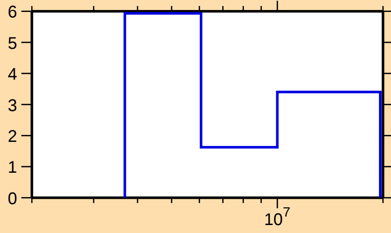
\Delta\sigma/\sigma vs. E for ^{139}\text{Cs}(n,\text{tot.})
