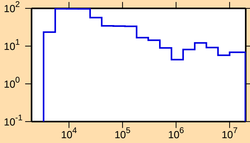
\Delta\sigma/\sigma vs. E for ^{139}\text{Cs}(n,\text{el.})
