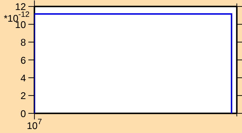
\sigma vs. E for ^{139}\text{Cs}(n,p\alpha)
