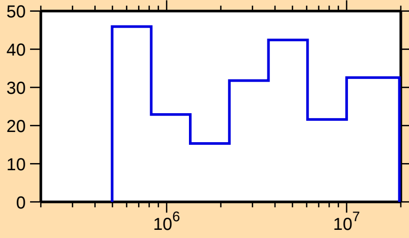
\Delta\sigma/\sigma vs. E for ^{139}\text{Cs}(n,n_1)
