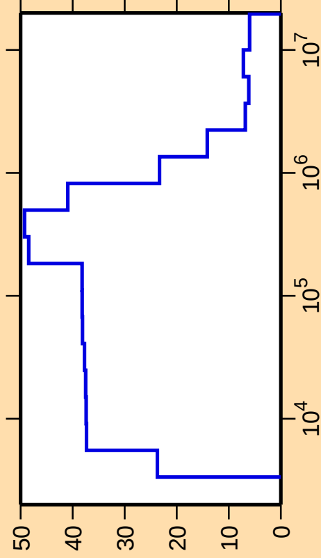
\Delta\sigma/\sigma vs. E for ^{139}\text{Cs}(n,\text{nonel.})
