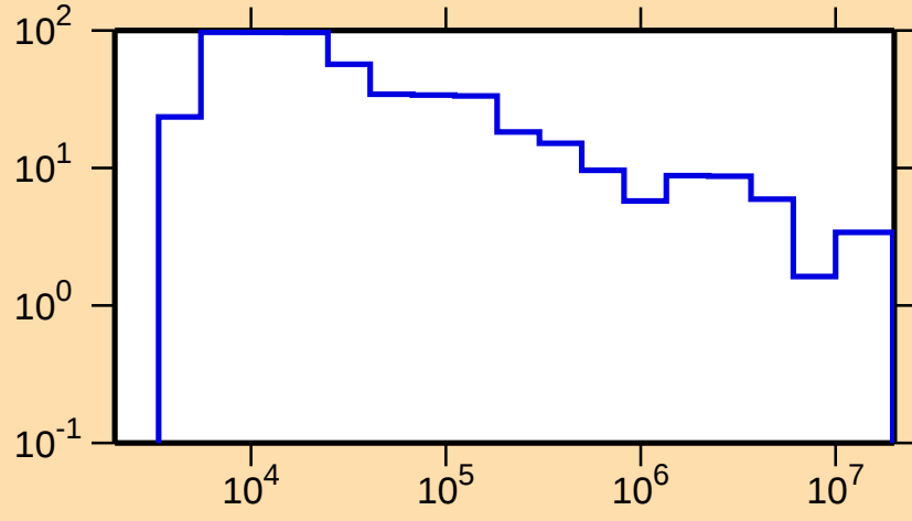
\Delta\sigma/\sigma vs. E for ^{139}\text{Cs}(n,\text{tot.})
