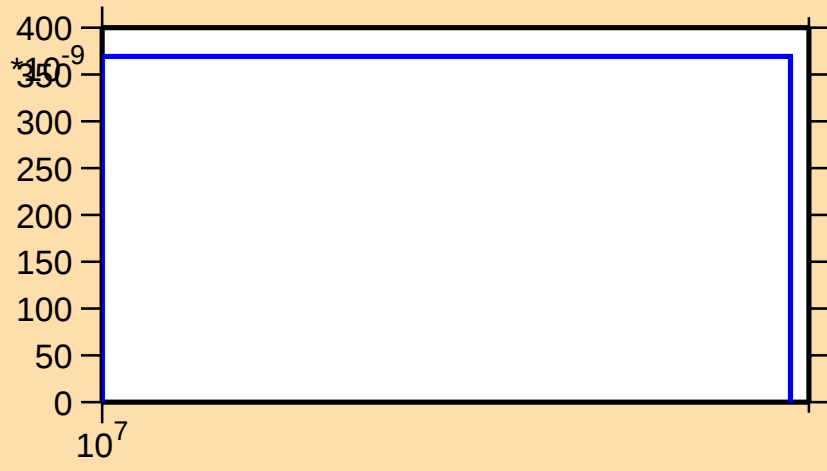
\sigma vs. E for ^{139}\text{Cs}(n,\text{nd})
