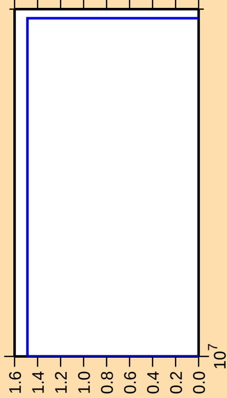
\Delta\sigma/\sigma vs. E for ^{139}\text{Cs} (mt 11)
