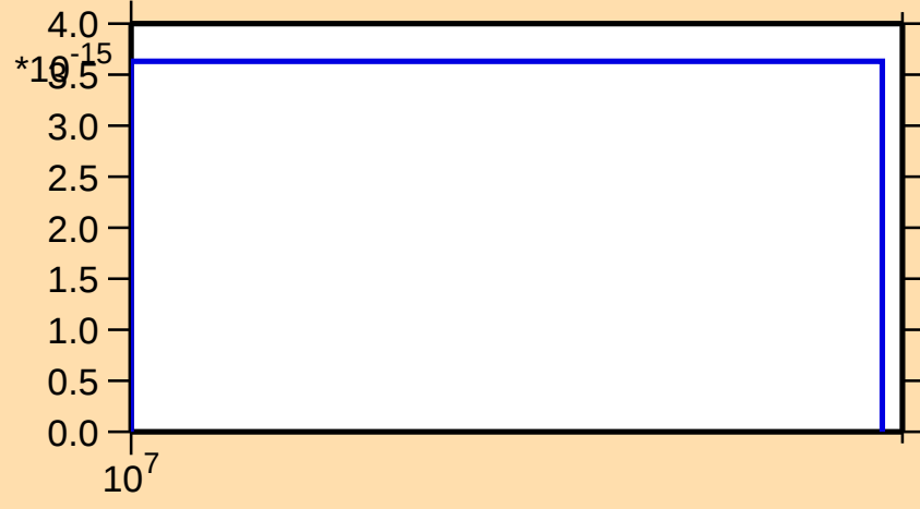
\sigma vs. E for ^{139}\text{Cs} (mt 45)
