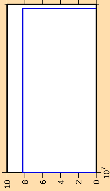
\Delta\sigma/\sigma vs. E for ^{139}\text{Cs}(n,3n)
