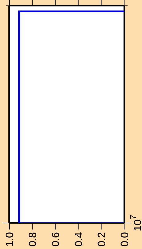
\Delta\sigma/\sigma vs. E for ^{139}\text{Cs}(\text{mt117})
