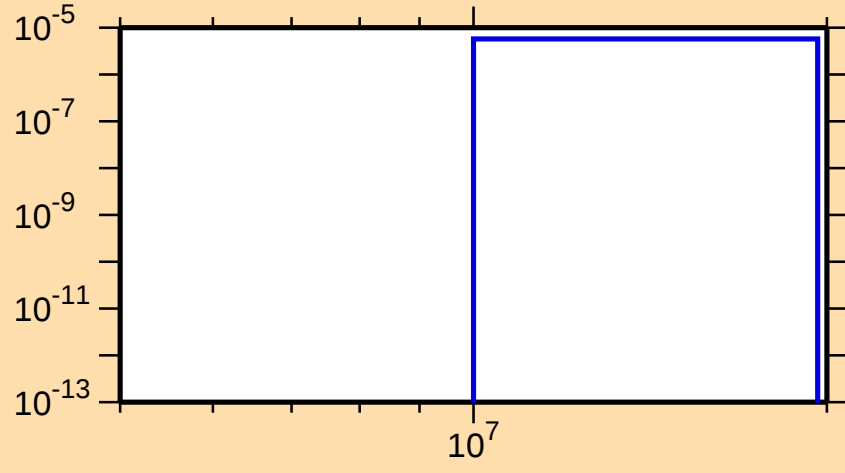
\sigma vs. E for ^{139}\text{Cs}(n,nt)
