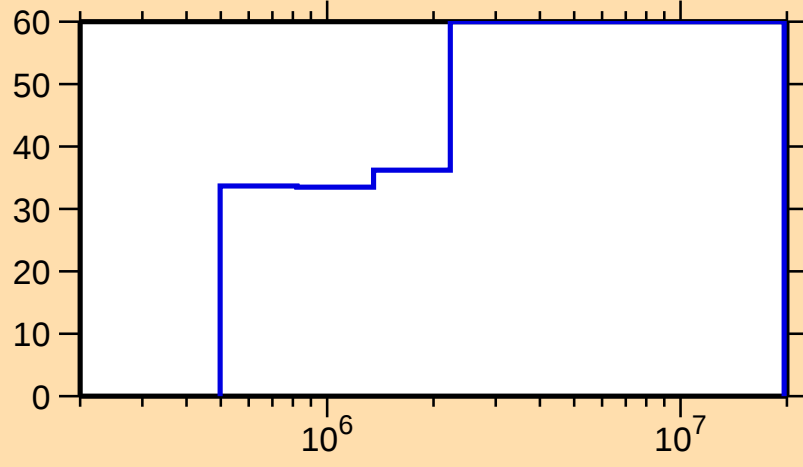
\Delta\sigma/\sigma vs. E for ^{139}\text{Cs}(n,\gamma)
