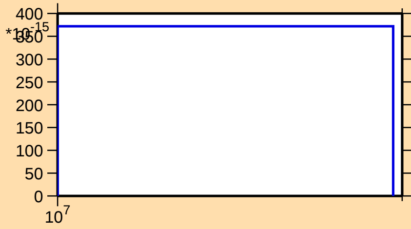
\sigma vs. E for ^{139}\text{Cs} (mt 11)
