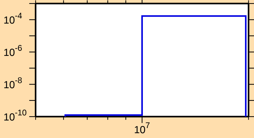
\sigma vs. E for ^{139}\text{Cs}(n,t)
