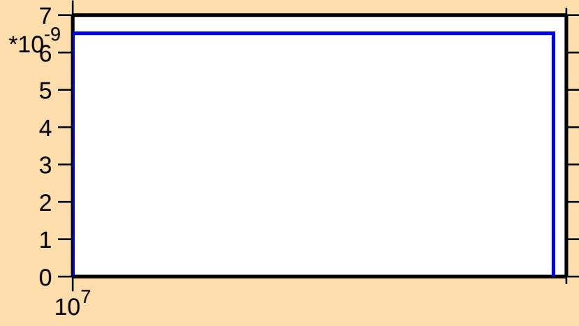
\sigma vs. E for ^{139}\text{Cs}(n,2np)
