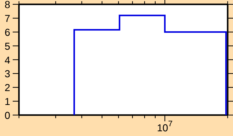
\Delta\sigma/\sigma vs. E for ^{139}\text{Cs}(n,\text{nonel.})
