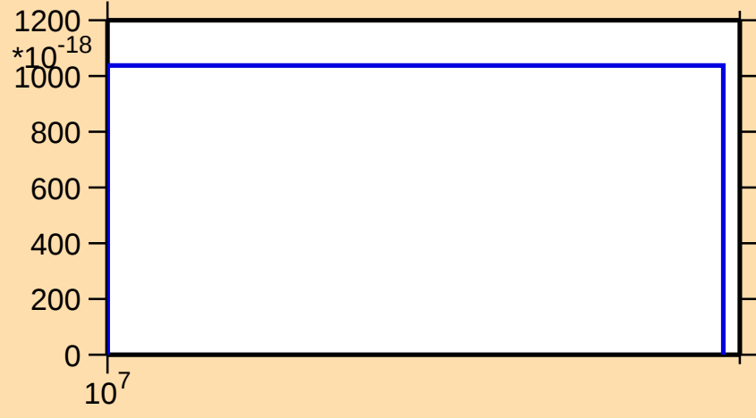
\sigma vs. E for ^{139}\text{Cs}(n,3n\alpha)
