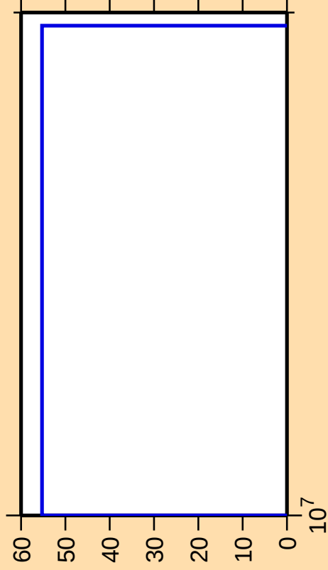
\Delta\sigma/\sigma vs. E for ^{139}\text{Cs}(n,p\alpha)
