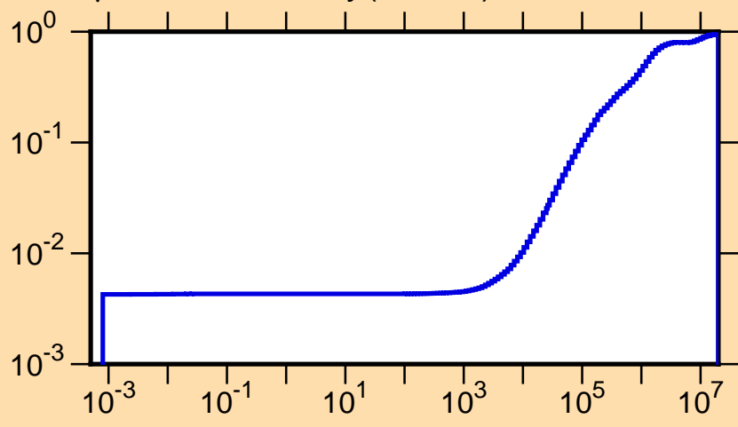
\mu vs. E for ^{158}\text{Dy}(\text{mt251})
