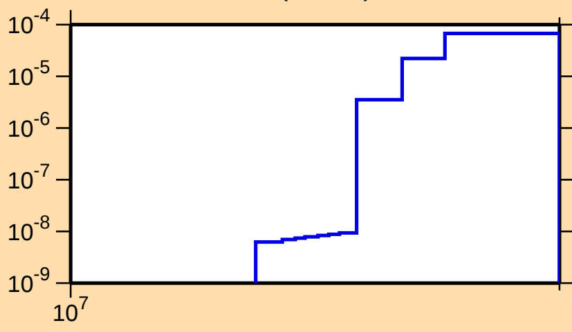
\sigma vs. E for ^{150}\text{Er}(n,2n\alpha)
