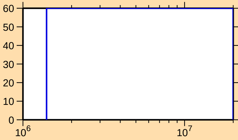
\Delta\sigma/\sigma vs. E for ^{150}\text{Er}(n,n_1)
