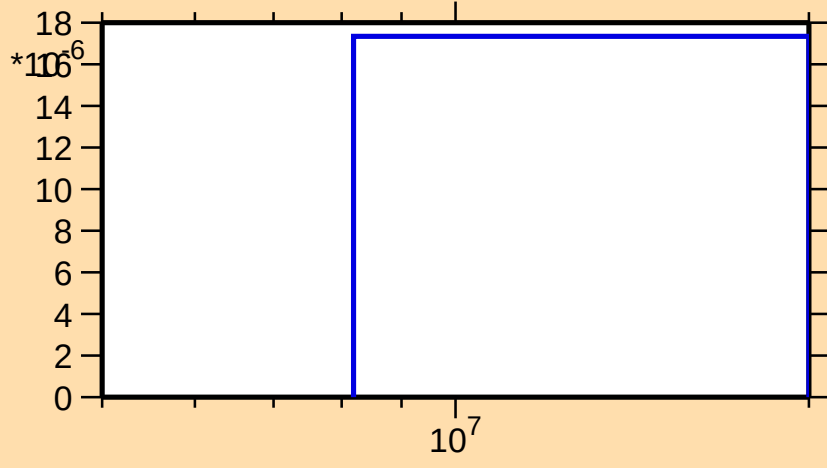
\sigma vs. E for ^{150}\text{Er}(n,t)
