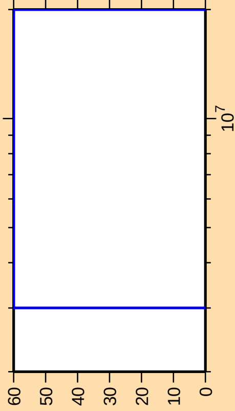
\Delta\sigma/\sigma vs. E for ^{150}\text{Er}(n,\text{ncont.})
