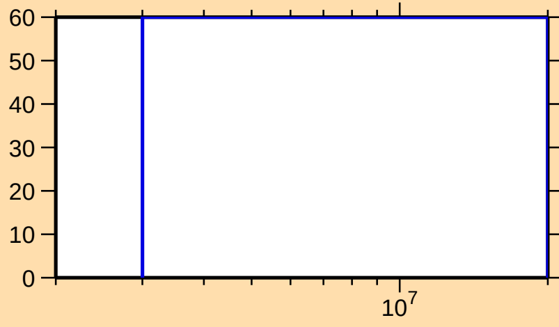
\Delta\sigma/\sigma vs. E for ^{150}\text{Er}(n,\text{ncont.})
