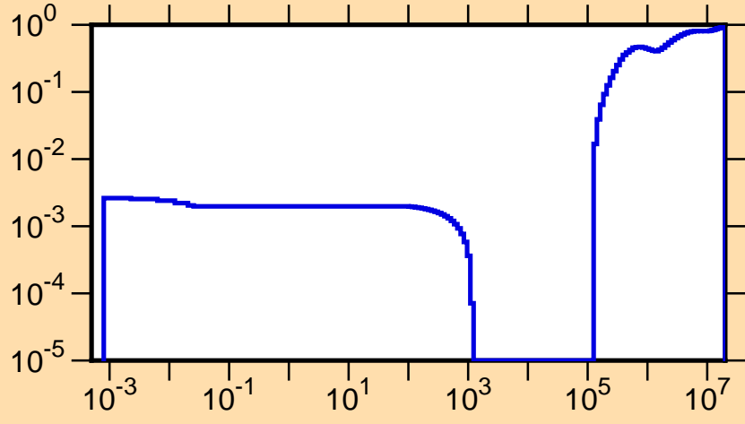
\mu vs. E for ^{252}\text{Es}(\text{mt251})
