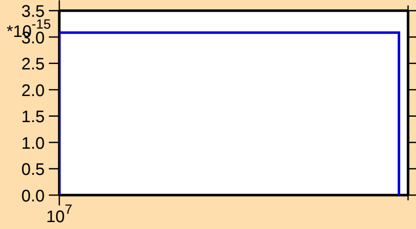
\sigma vs. E for ^{252}\text{Es}(\text{mt } 42)
