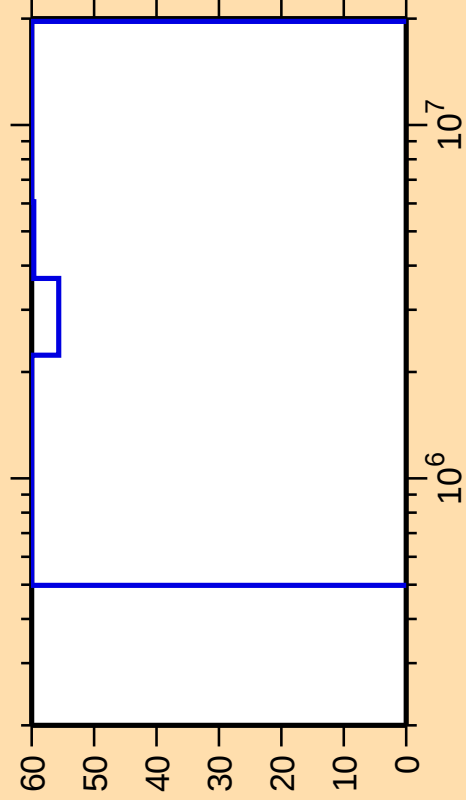
\Delta\sigma/\sigma vs. E for ^{252}\text{Es}(n,n_{\text{cont}})
