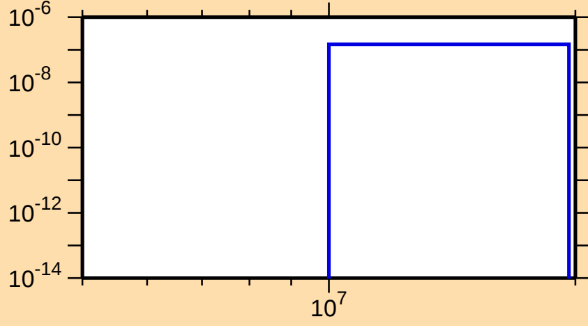
\sigma vs. E for ^{252}\text{Es}(n,2np)
