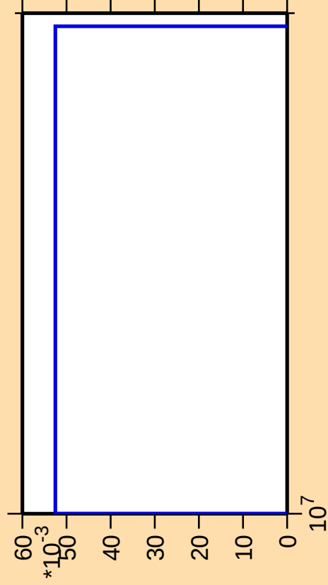
\Delta\sigma/\sigma vs. E for ^{252}\text{Es}(\text{mt 11})
