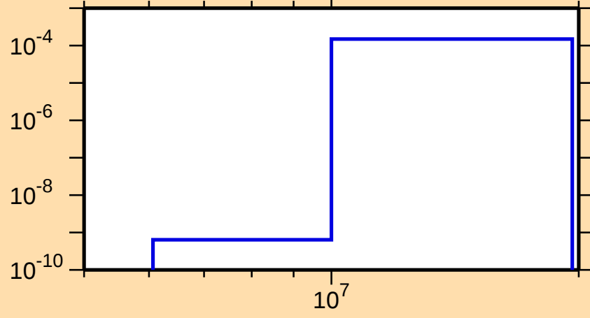
\sigma vs. E for ^{252}\text{Es}(n,t)
