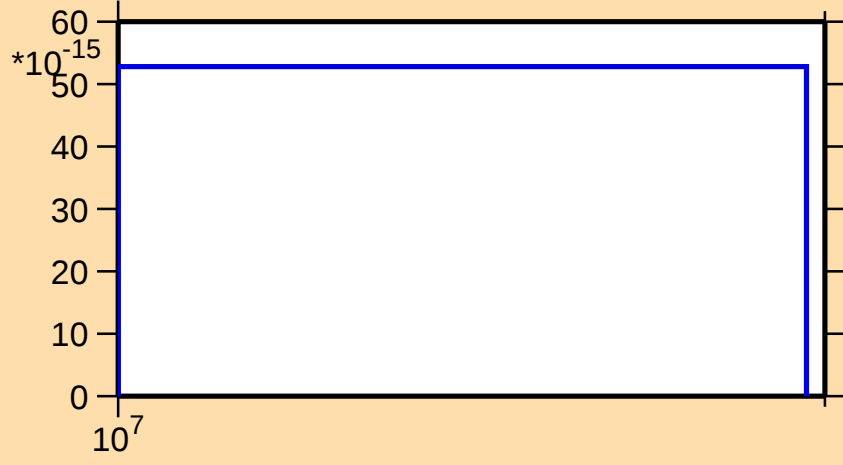
\sigma vs. E for ^{252}\text{Es}(\text{mt 11})
