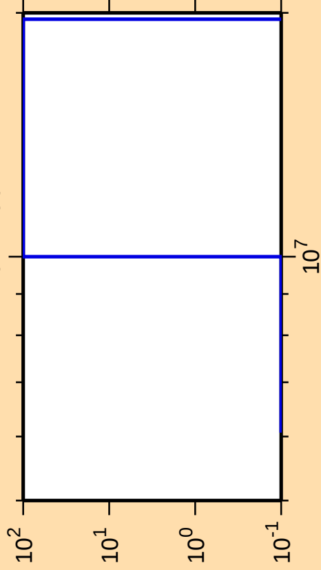
\Delta\sigma/\sigma vs. E for ^{252}\text{Es}(n,2np)
