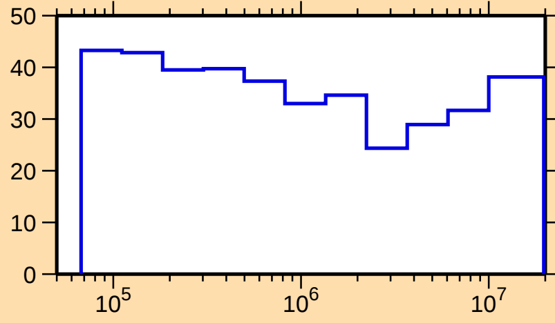
\Delta\sigma/\sigma vs. E for ^{252}\text{Es}(n,\text{el.})
