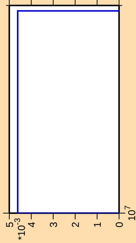
\Delta\sigma/\sigma vs. E for ^{252}\text{Es}(\text{mt } 34)
