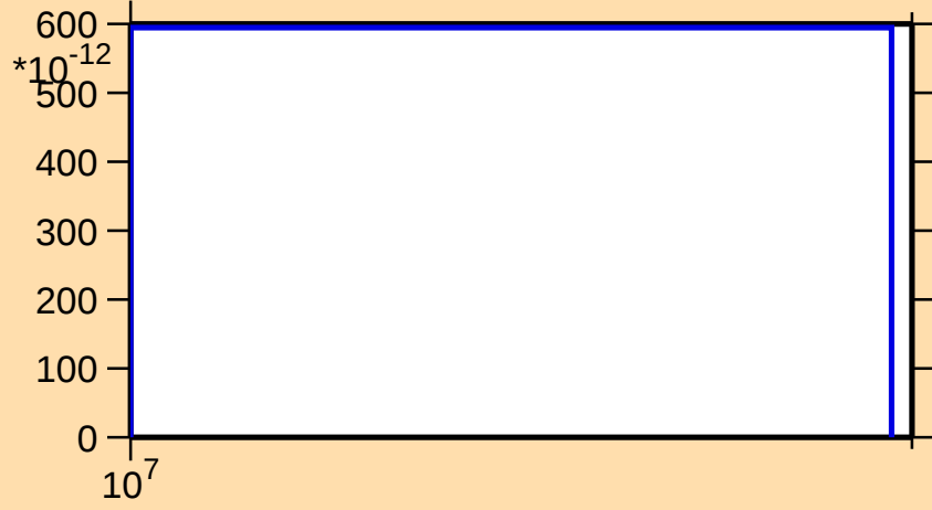
\sigma vs. E for ^{252}\text{Es}(\text{mt } 45)
