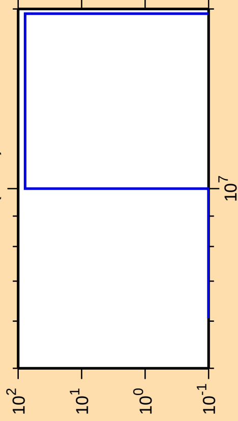
\Delta\sigma/\sigma vs. E for ^{252}\text{Es}(n,\text{nd})
