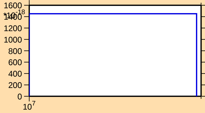
\sigma vs. E for ^{252}\text{Es}(\text{mt } 34)
