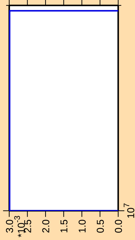
\Delta\sigma/\sigma vs. E for ^{252}\text{Es}(\text{mt } 42)
