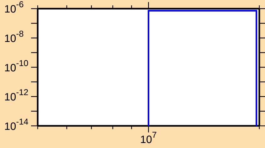
\sigma vs. E for ^{252}\text{Es}(n,\text{nd})
