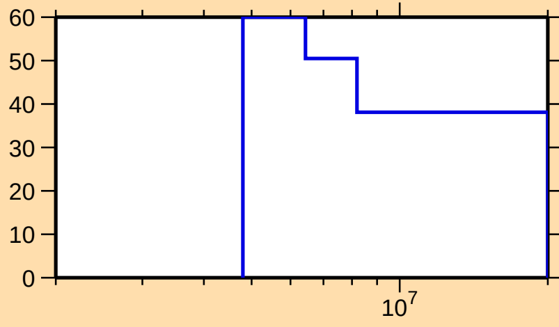
\Delta\sigma/\sigma vs. E for ^{252}\text{Es}(n,2n)
