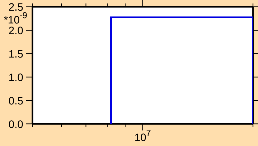
\sigma vs. E for ^{252}\text{Es}(\text{mt117})
