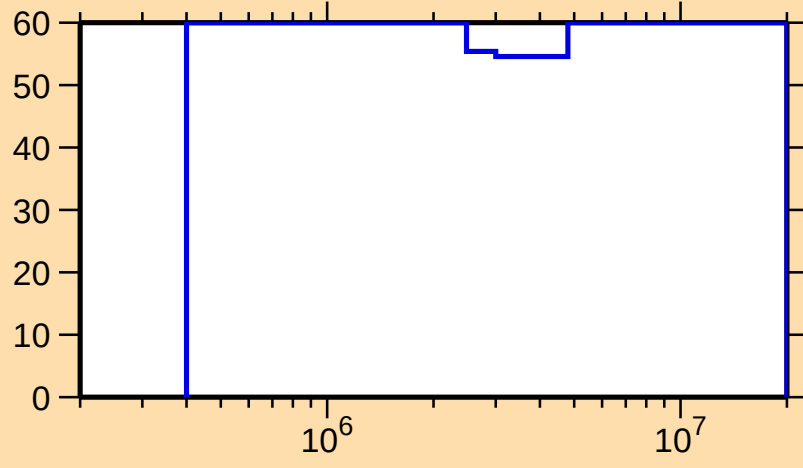
\Delta\sigma/\sigma vs. E for ^{252}\text{Es}(n,n\text{cont.})
