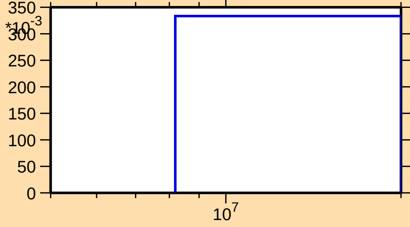
\sigma vs. E for ^{252}\text{Es}(n,3n)
