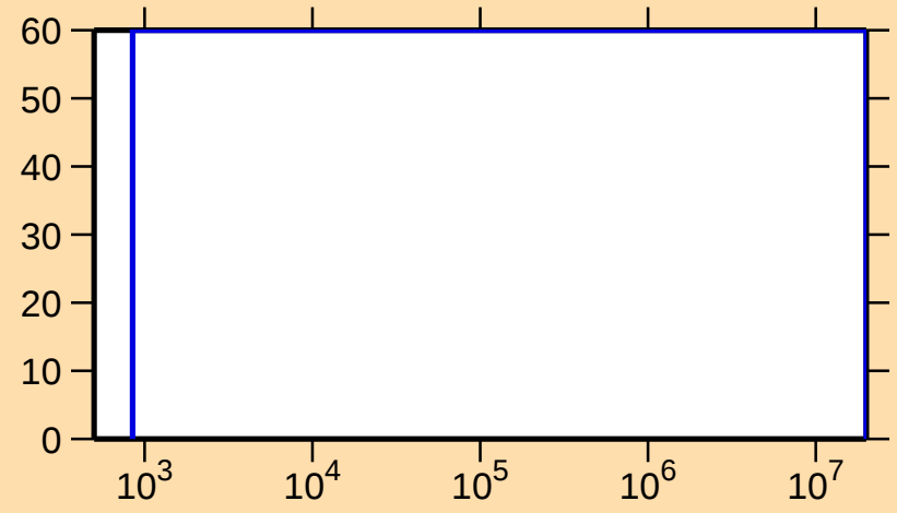
\Delta\sigma/\sigma vs. E for ^{256}\text{Es}(n,\gamma)
