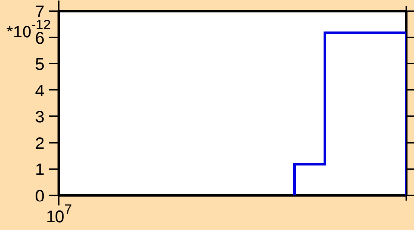
\sigma vs. E for ^{256}\text{Es}(\text{mt } 45)
