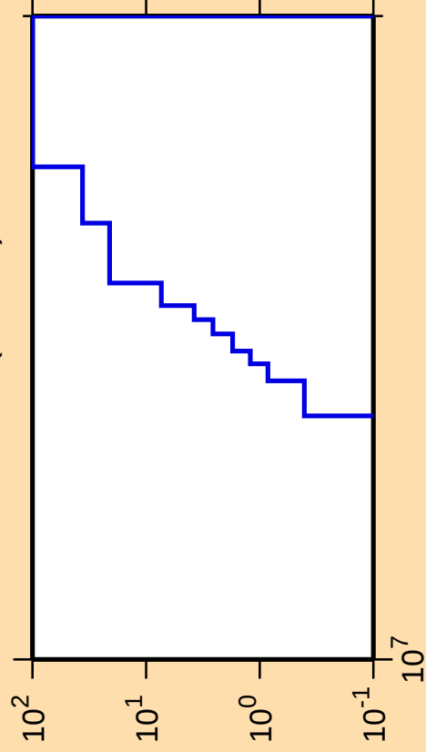
\Delta\sigma/\sigma vs. E for ^{256}\text{Es}(\text{mt117})
