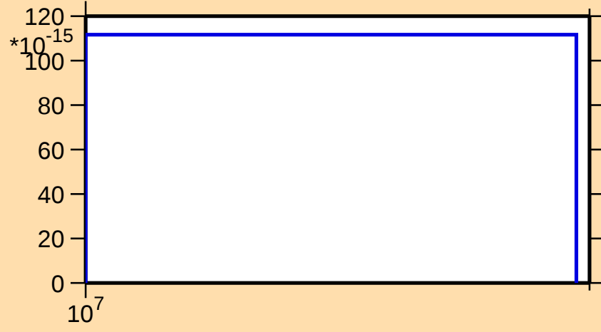
\sigma vs. E for ^{256}\text{Es}(\text{mt 11})
