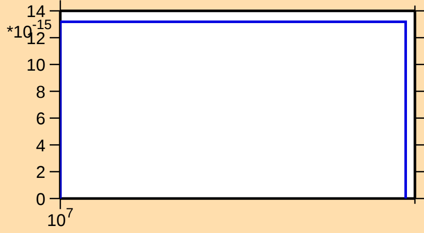
\sigma vs. E for ^{256}\text{Es}(\text{mt } 42)
