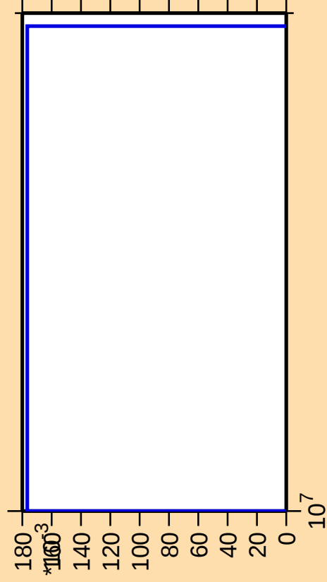
\Delta\sigma/\sigma vs. E for ^{256}\text{Es}(\text{mt 11})
