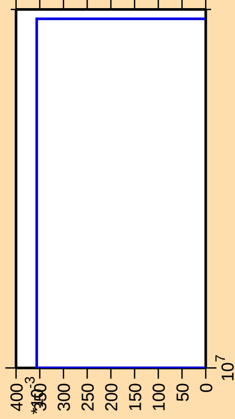
\Delta\sigma/\sigma vs. E for ^{256}\text{Es}(\text{mt } 45)
