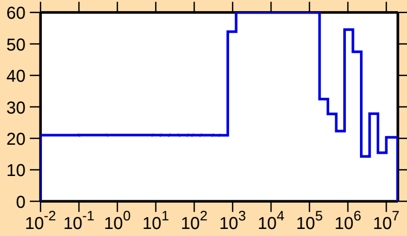
\Delta\sigma/\sigma vs. E for ^{256}\text{Es}(n,el.)
