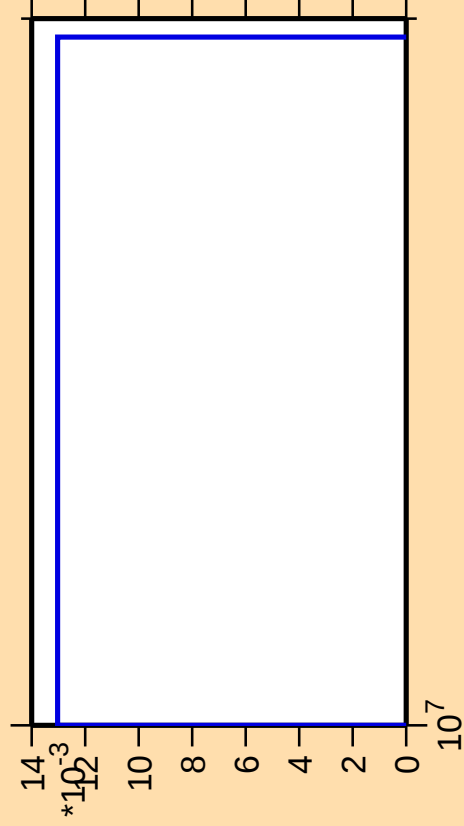
\Delta\sigma/\sigma vs. E for ^{256}\text{Es}(\text{mt } 42)
