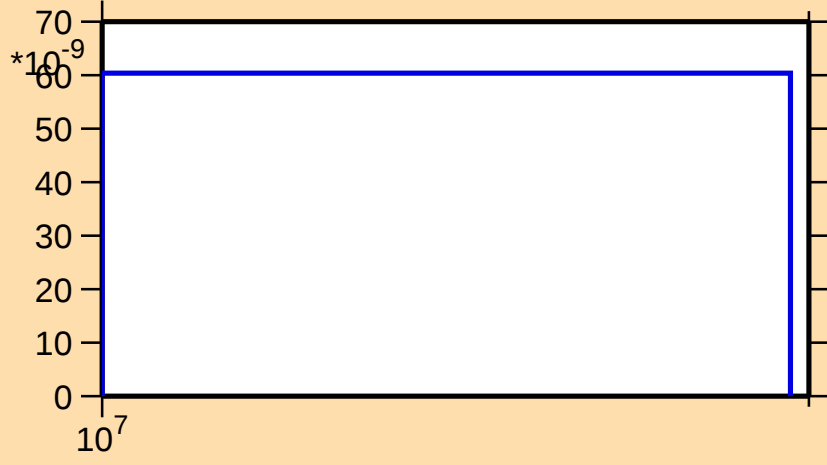
\sigma vs. E for ^{256}\text{Es}(n,2np)
