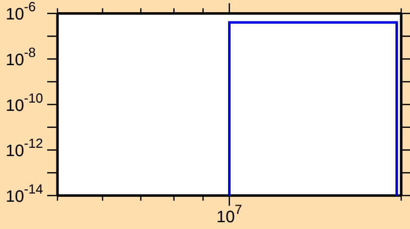
\sigma vs. E for ^{256}\text{Es}(n,nd)
