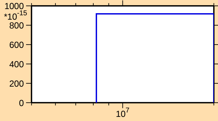
\sigma vs. E for ^{256}\text{Es}(\text{mt117})
