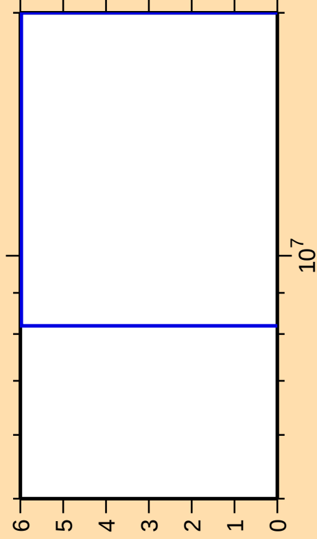
\Delta\sigma/\sigma vs. E for ^{256}\text{Es}(\text{mt117})
