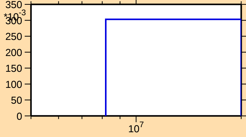
\sigma vs. E for ^{256}\text{Es}(n,3n)
