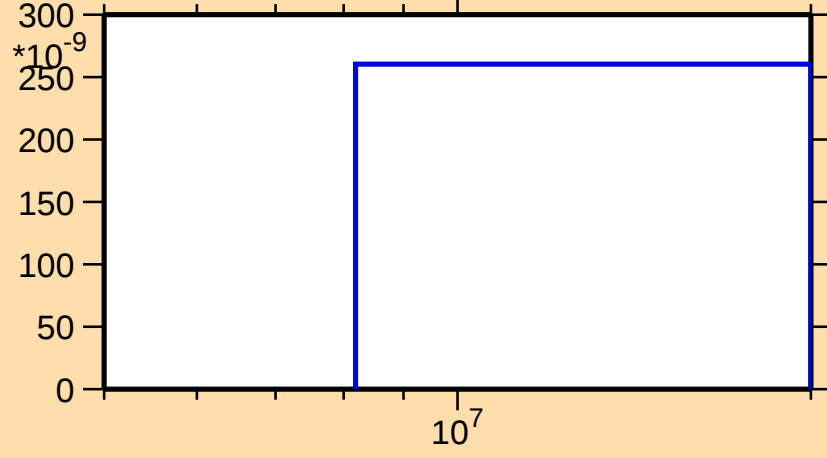
\sigma vs. E for ^{256}\text{Es}(n,nt)
