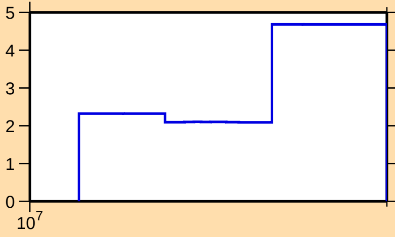
\Delta\sigma/\sigma vs. E for ^{141}\text{Eu}(n,\text{tot.})
