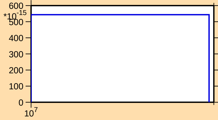
\sigma vs. E for ^{141}\text{Eu} (mt 34)
