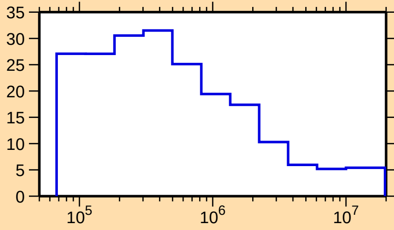
\Delta\sigma/\sigma vs. E for ^{141}\text{Eu}(n, \text{nonel.})
