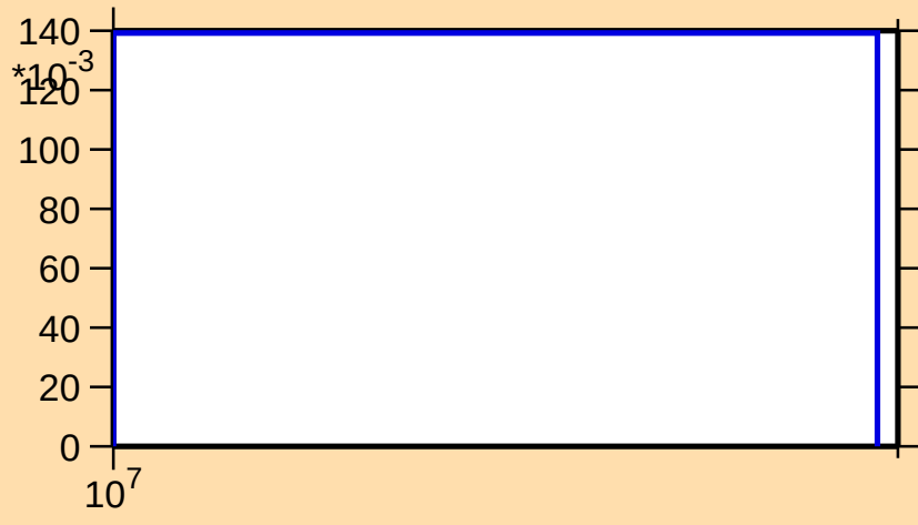
\sigma vs. E for ^{141}\text{Eu}(n,2n)
