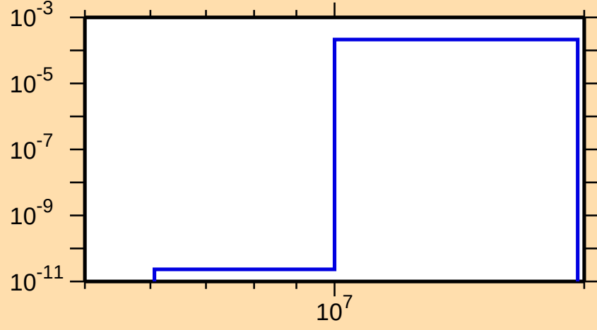
\sigma vs. E for ^{141}\text{Eu}(n,t)
