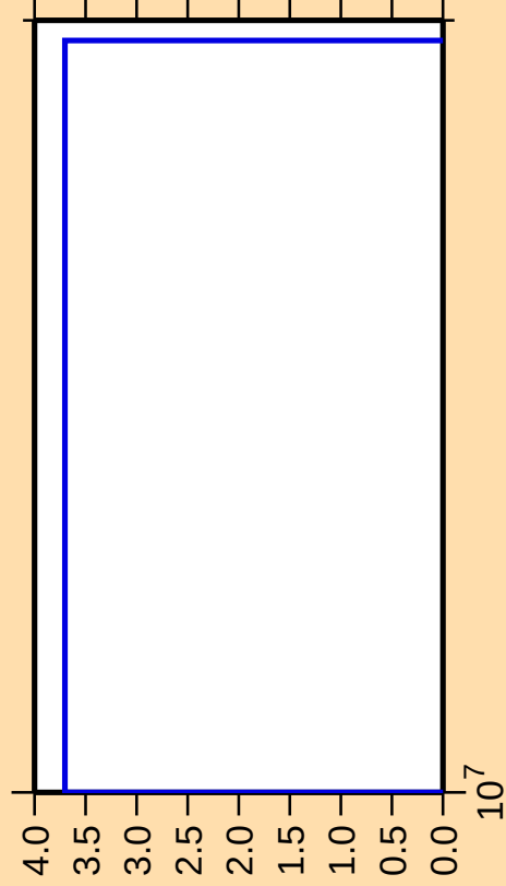
\Delta\sigma/\sigma vs. E for ^{141}\text{Eu} (mt 34)
