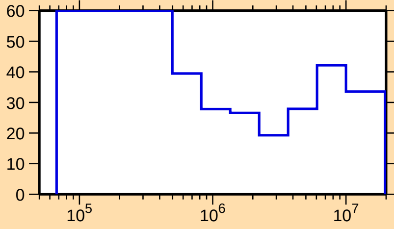
\Delta\sigma/\sigma vs. E for ^{141}\text{Eu}(n,n_1)
