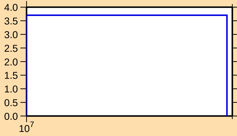
\Delta\sigma/\sigma vs. E for ^{141}\text{Eu}(n,\text{el.})
