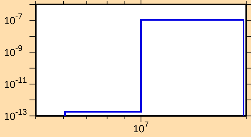
\sigma vs. E for ^{141}\text{Eu}(\text{mt117})
