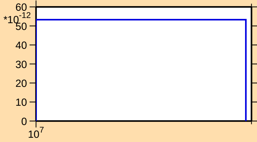
\sigma vs. E for ^{141}\text{Eu}(n,\text{pt})
