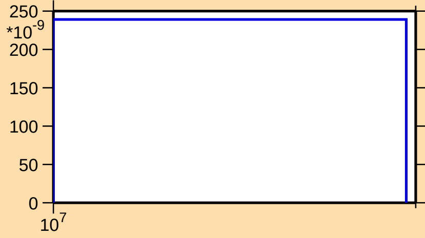
\sigma vs. E for ^{141}\text{Eu}(n,\text{nd})
