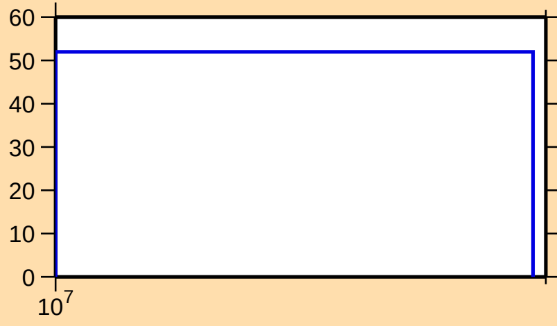
\Delta\sigma/\sigma vs. E for ^{141}\text{Eu}(n,2n)
