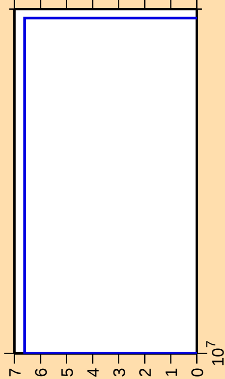
\Delta\sigma/\sigma vs. E for ^{144}\text{Eu}(n,nt)
