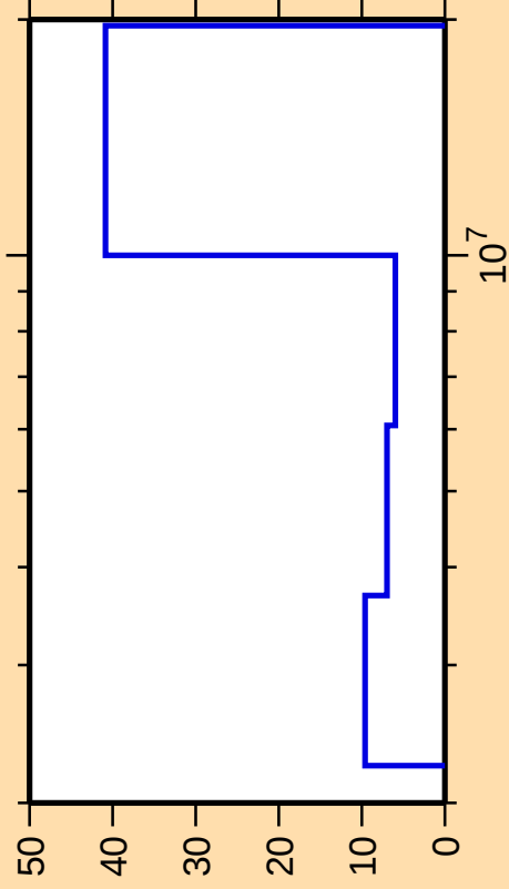
\Delta\sigma/\sigma vs. E for ^{144}\text{Eu}(\text{n},\text{ncont.})
