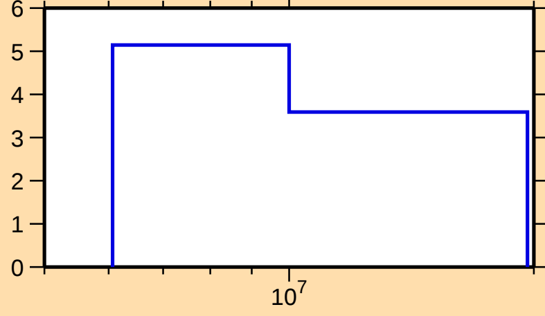
\Delta\sigma/\sigma vs. E for ^{144}\text{Eu}(n,\text{el.})
