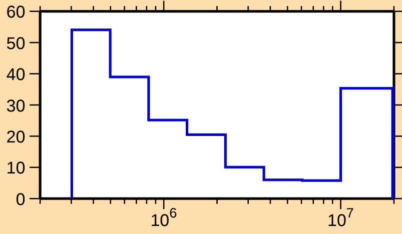
\Delta\sigma/\sigma vs. E for ^{144}\text{Eu}(n,\text{inel.})
