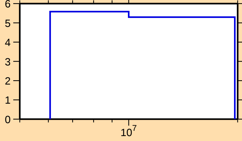
\Delta\sigma/\sigma vs. E for ^{144}\text{Eu}(n,\text{nonel.})
