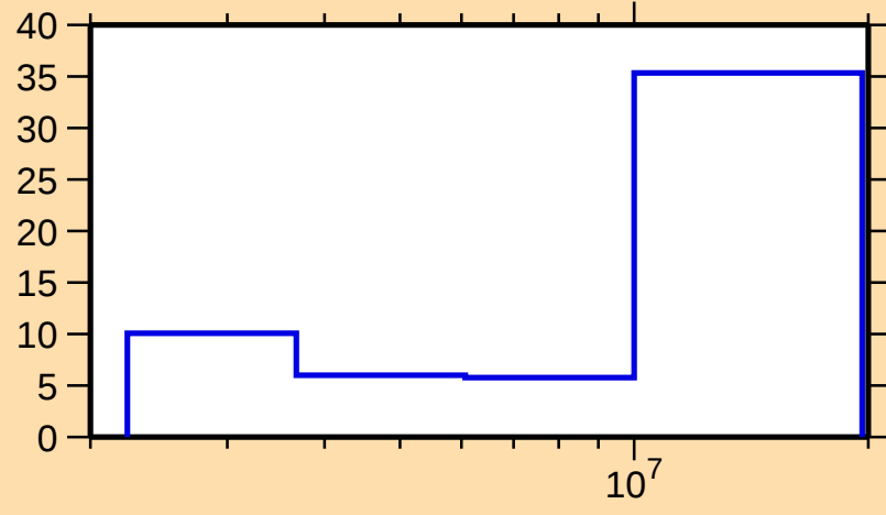
\Delta\sigma/\sigma vs. E for ^{144}\text{Eu}(\text{n},\text{inel.})
