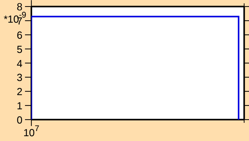
\sigma vs. E for ^{144}\text{Eu}(n,\text{pd})
