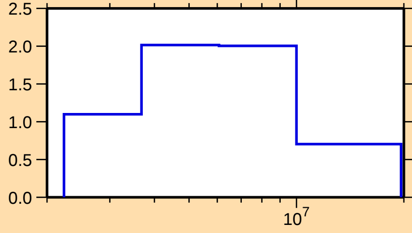
\sigma vs. E for ^{144}\text{Eu}(n,n\text{cont.})
