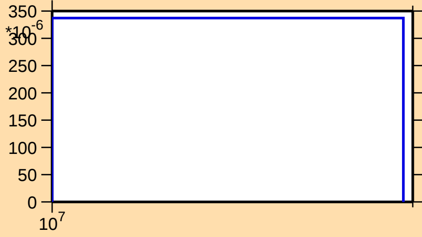
\sigma vs. E for ^{144}\text{Eu}(n,2np)
