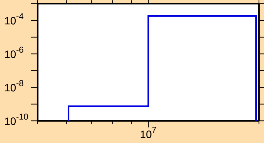
\sigma vs. E for ^{144}\text{Eu}(n,t)
