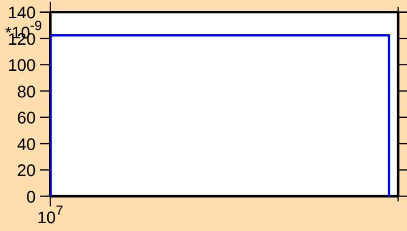
\sigma vs. E for ^{144}\text{Eu}(n,2n\alpha)
