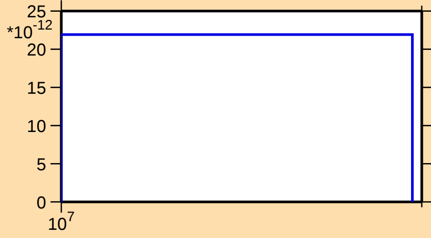
\sigma vs. E for ^{144}\text{Eu}(n,\text{pt})
