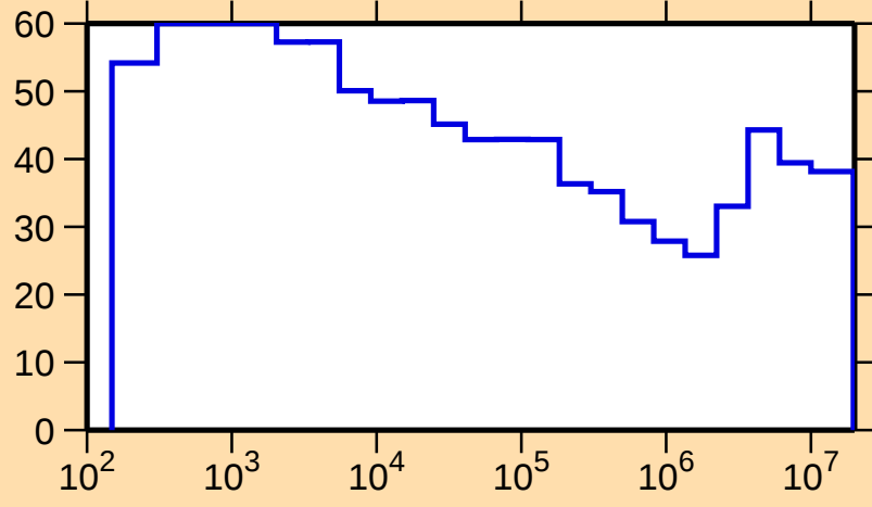
\Delta\sigma/\sigma vs. E for ^{144}\text{Eu}(n,p)
