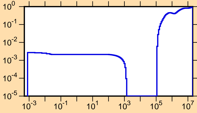
\mu vs. E for ^{245}\text{Fm}(\text{mt251})
