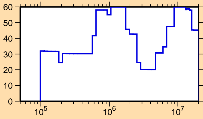
\Delta\sigma/\sigma vs. E for ^{245}\text{Fm}(n,el.)
