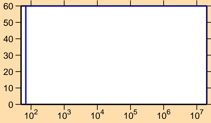
\Delta\sigma/\sigma vs. E for ^{245}\text{Fm}(n,\gamma)
