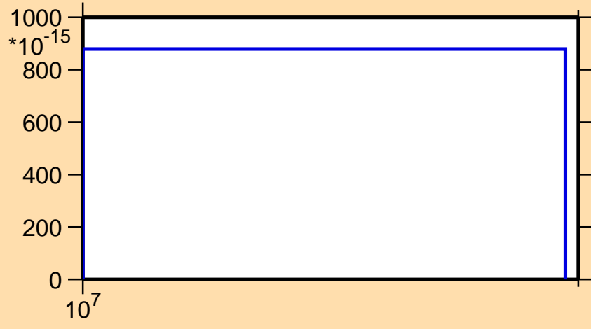
\sigma vs. E for ^{245}\text{Fm} (mt 34)
