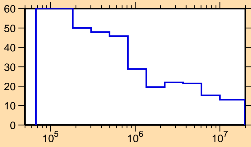
\Delta\sigma/\sigma vs. E for ^{245}\text{Fm}(n, nonel.)
