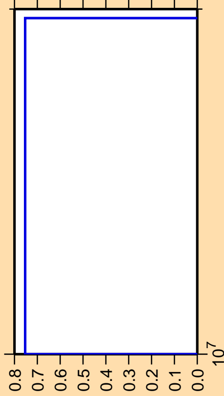
\Delta\sigma/\sigma vs. E for ^{245}\text{Fm} (mt 34)
