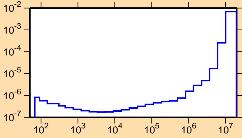
\sigma vs. E for ^{245}\text{Fm}(n,p\alpha)
