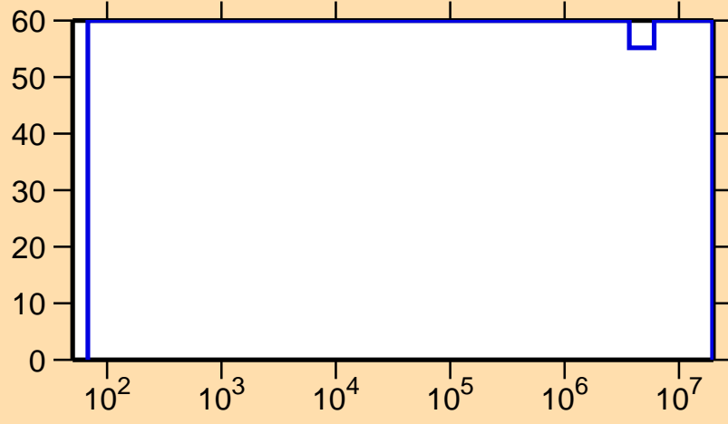
\Delta\sigma/\sigma vs. E for ^{245}\text{Fm}(n,p)
