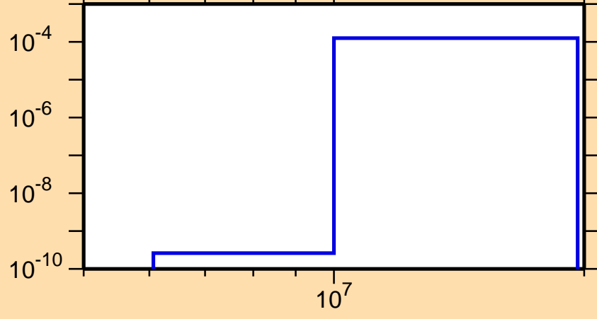
\sigma vs. E for ^{245}\text{Fm}(n,t)
