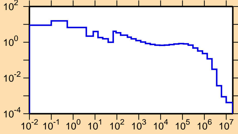
\sigma vs. E for ^{245}\text{Fm}(n,\gamma)
