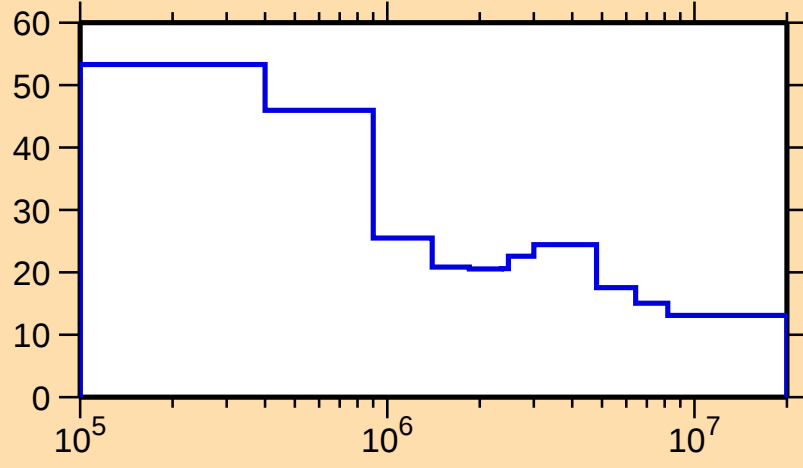
\Delta\sigma/\sigma vs. E for ^{245}\text{Fm}(n,\text{nonel.})
