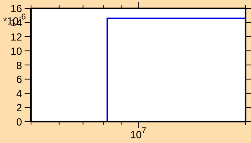
\sigma vs. E for ^{245}\text{Fm}(n,3n\alpha)
