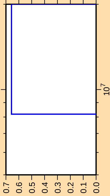
\Delta\sigma/\sigma vs. E for ^{245}\text{Fm}(\text{mt } 34)
