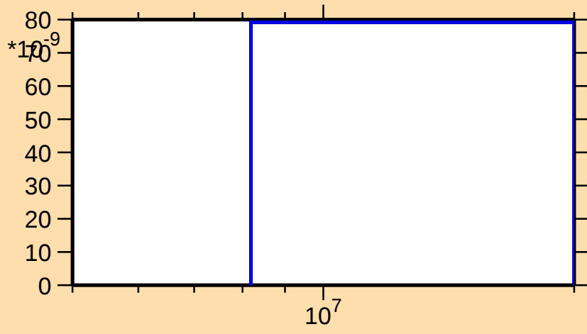
\sigma vs. E for ^{245}\text{Fm}(n,\text{nd})
