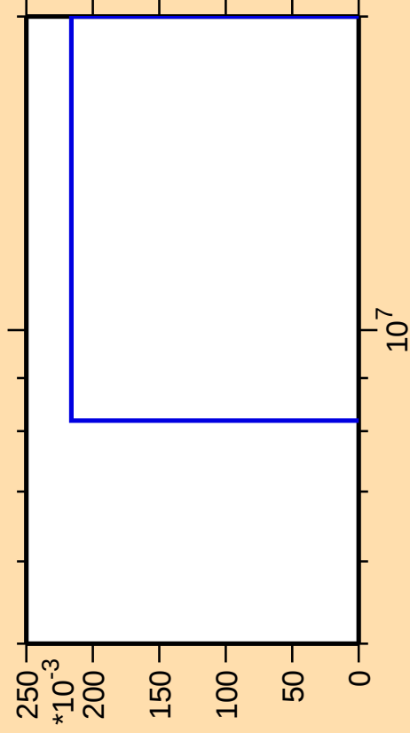
\Delta\sigma/\sigma vs. E for ^{245}\text{Fm}(n,\text{pt})
