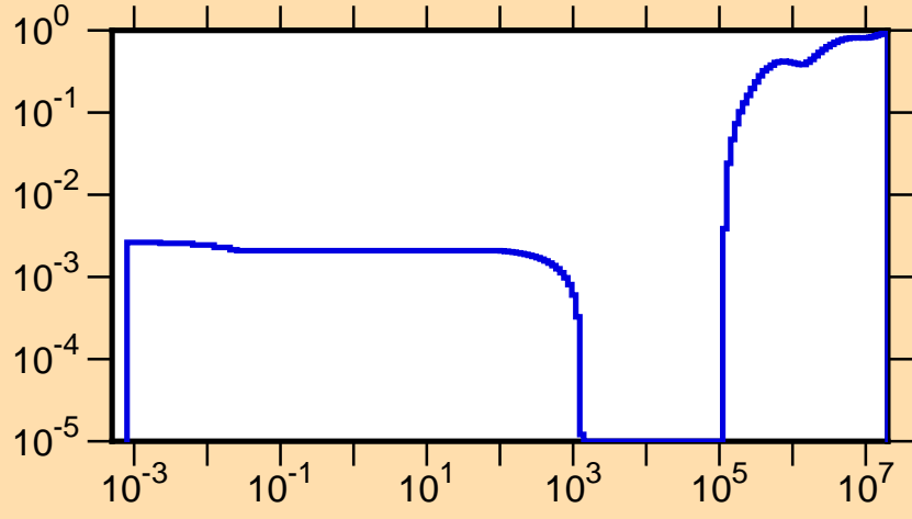
\mu vs. E for ^{252}\text{Fm}(\text{mt251})
