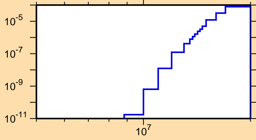
\sigma vs. E for ^{252}\text{Fm}(\text{mt117})
