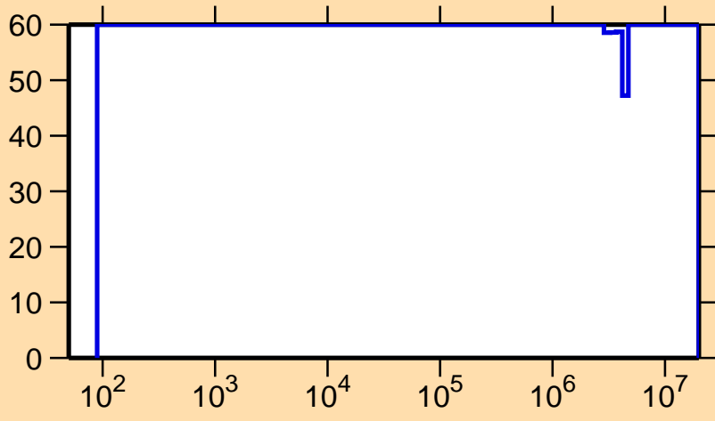
\Delta\sigma/\sigma vs. E for ^{252}\text{Fm}(n,\gamma)
