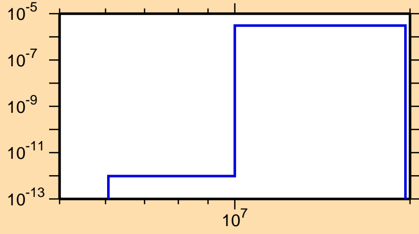
\sigma vs. E for ^{252}\text{Fm} (mt 45)
