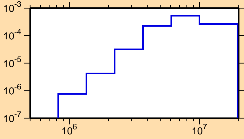
\sigma vs. E for ^{252}\text{Fm}(n,n\alpha)
