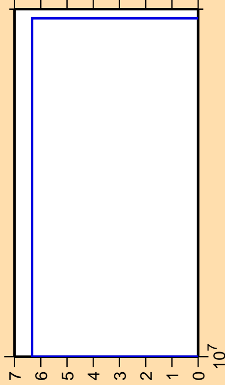
\Delta\sigma/\sigma vs. E for ^{252}\text{Fm}(n,\text{He3})
