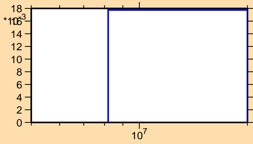
\sigma vs. E for ^{252}\text{Fm}(n,3n)
