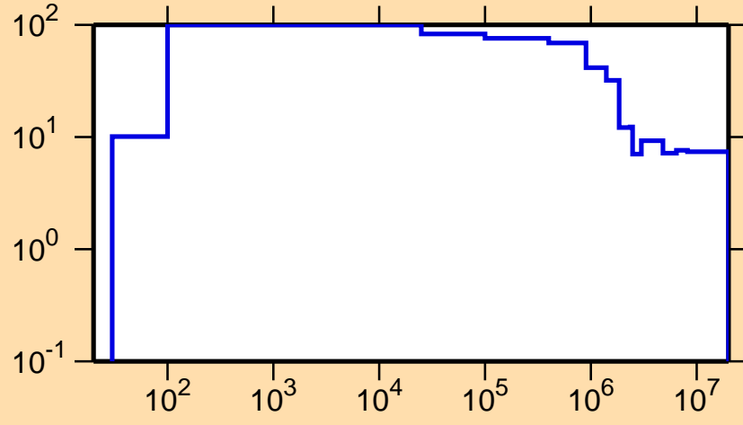
\Delta\sigma/\sigma vs. E for ^{252}\text{Fm}(n,\text{nonel.})
