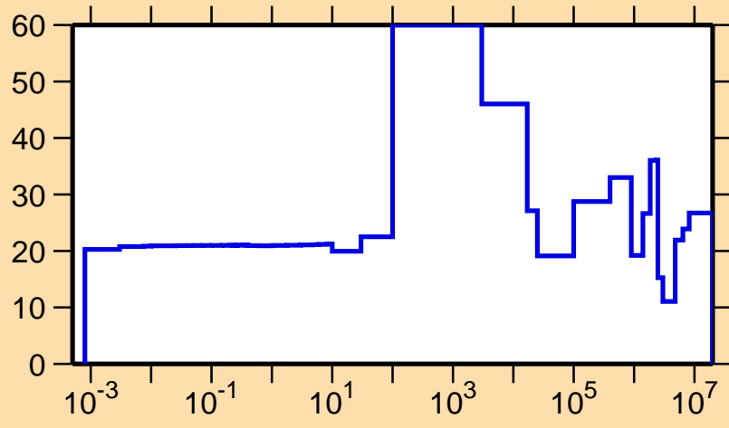
\Delta\sigma/\sigma vs. E for ^{252}\text{Fm}(n,\text{el.})
