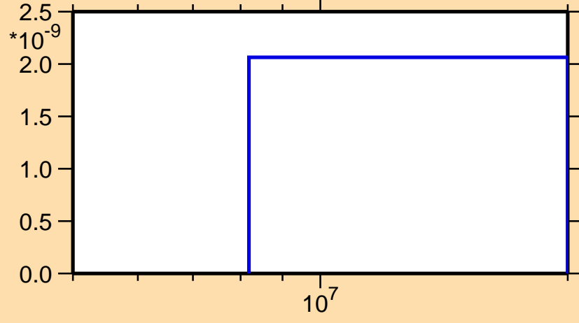
\sigma vs. E for ^{252}\text{Fm}(n,nt)
