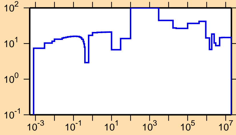
\Delta\sigma/\sigma vs. E for ^{252}\text{Fm}(n,\text{tot.})
