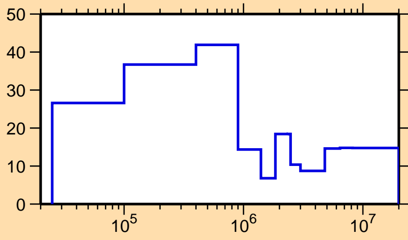
\Delta\sigma/\sigma vs. E for ^{252}\text{Fm}(n,\text{tot.})
