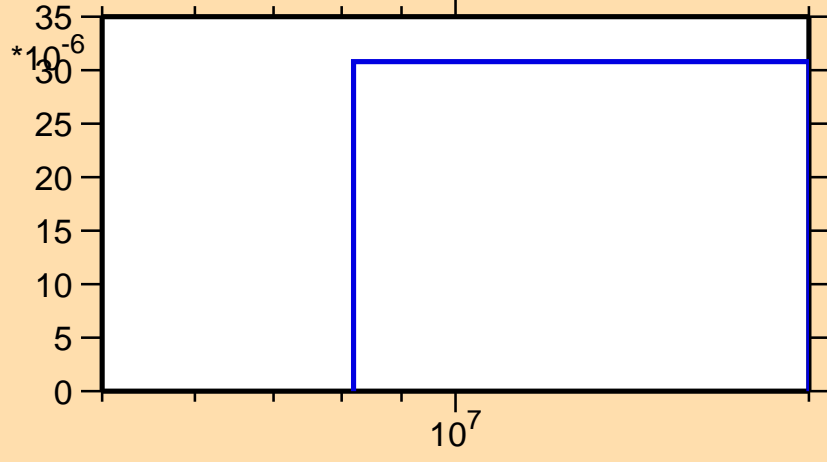
\sigma vs. E for ^{252}\text{Fm}(n,t)
