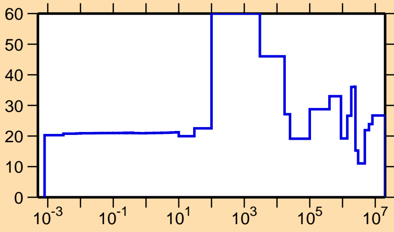
\Delta\sigma/\sigma vs. E for ^{252}\text{Fm}(n,el.)
