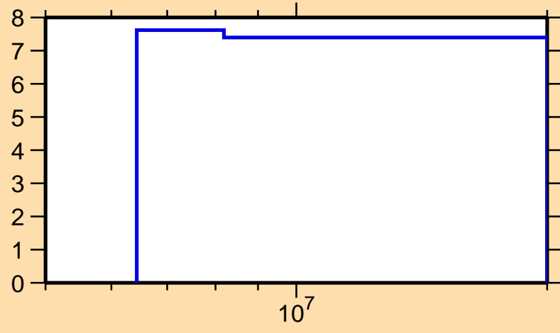
\Delta\sigma/\sigma vs. E for ^{252}\text{Fm}(n,\text{nonel.})
