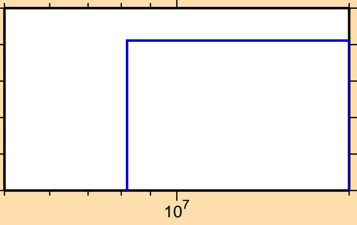
\sigma vs. E for ^{252}\text{Fm}(n,nd)
