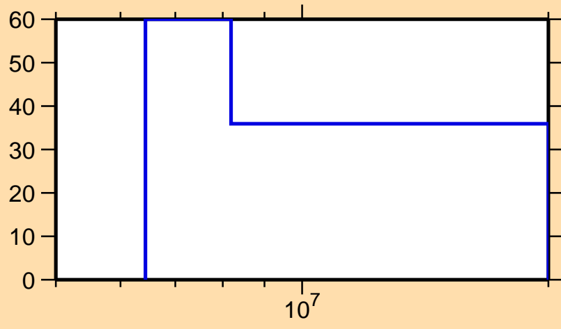
\Delta\sigma/\sigma vs. E for ^{252}\text{Fm}(n,2n)
