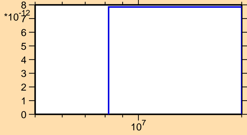
\sigma vs. E for ^{252}\text{Fm}(n,\text{He}3)
