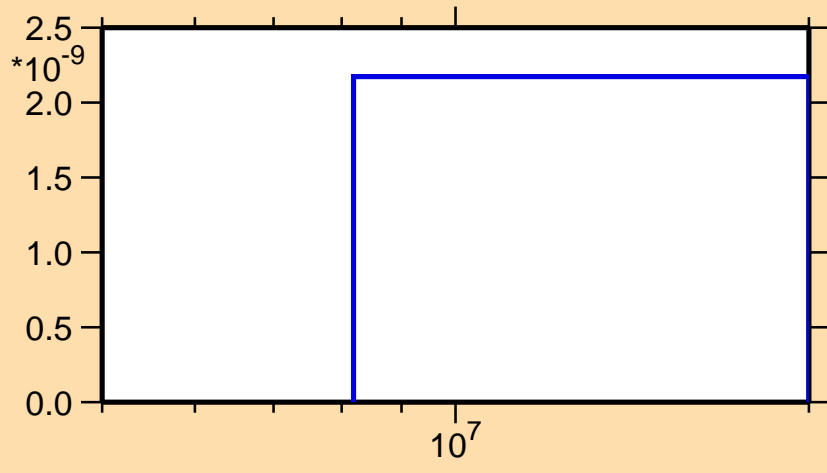
\sigma vs. E for ^{252}\text{Fm}(n,2np)
