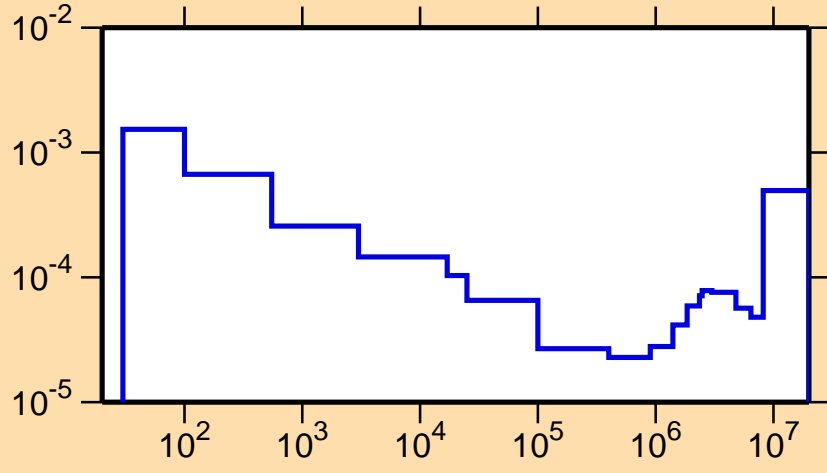
\sigma vs. E for ^{252}\text{Fm}(n,\alpha)
