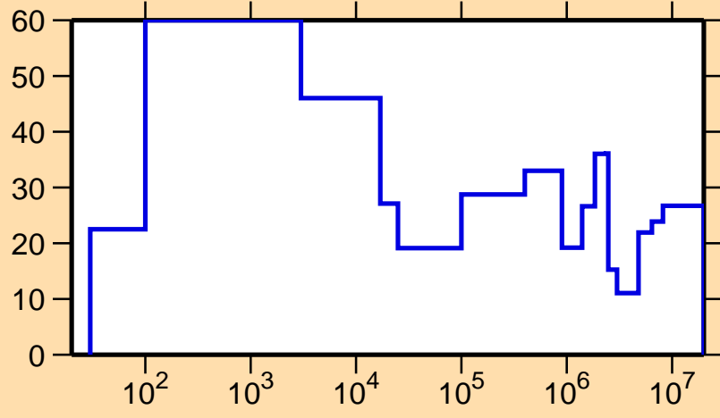
\Delta\sigma/\sigma vs. E for ^{252}\text{Fm}(n,\text{el.})
