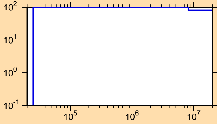
\Delta\sigma/\sigma vs. E for ^{252}\text{Fm}(n,f)
