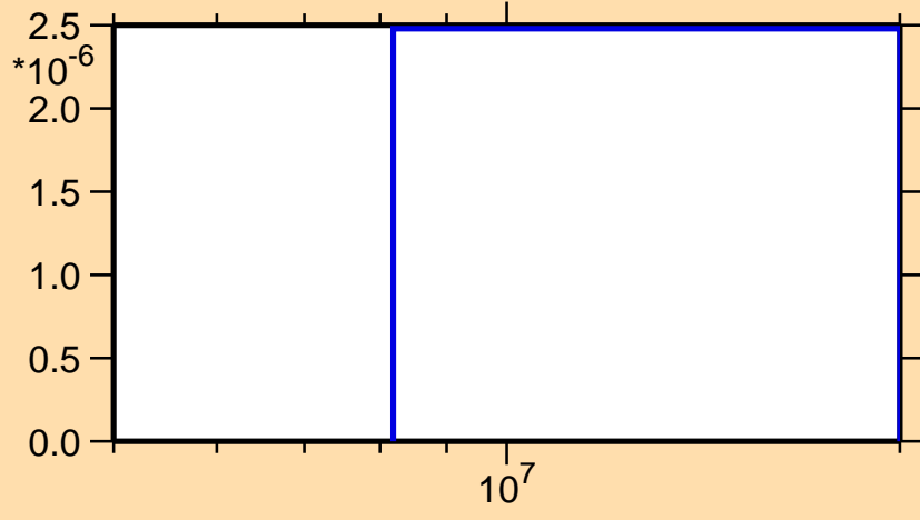
\sigma vs. E for ^{252}\text{Fm} (mt 45)
