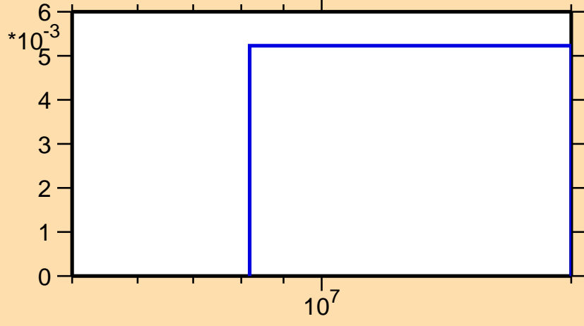
\sigma vs. E for ^{252}\text{Fm}(n,3n\alpha)
