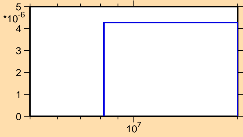
\sigma vs. E for ^{252}\text{Fm}(\text{mt117})
