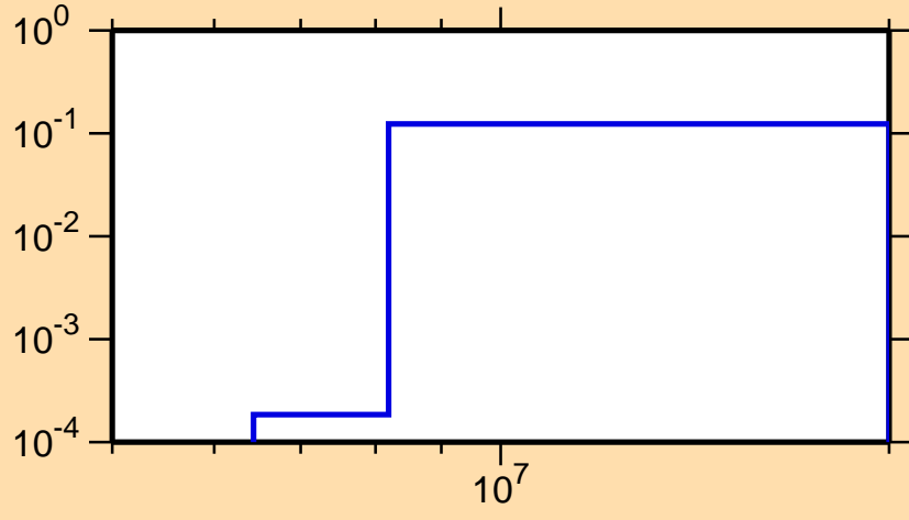
\sigma vs. E for ^{252}\text{Fm}(n,2n\alpha)
