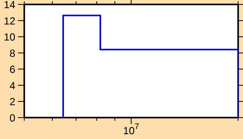
\Delta\sigma/\sigma vs. E for ^{260}\text{Fm}(n,\text{tot.})
