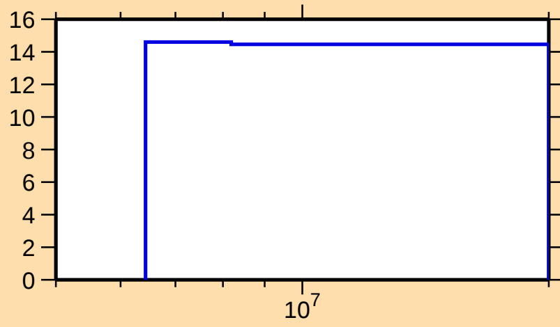
\Delta\sigma/\sigma vs. E for ^{260}\text{Fm}(n,\text{nonel.})
