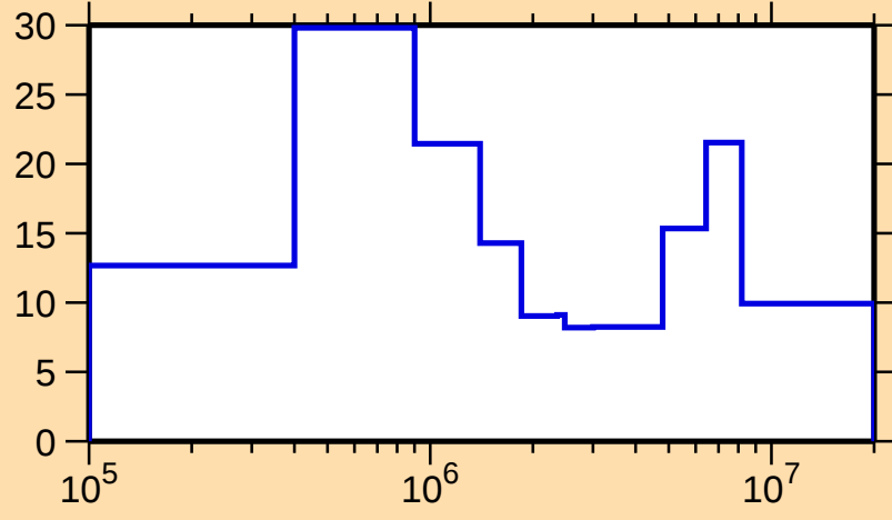
\Delta\sigma/\sigma vs. E for ^{260}\text{Fm}(n,\text{el.})
