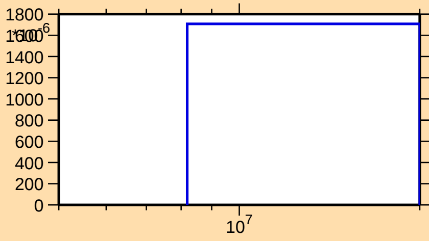
\sigma vs. E for ^{260}\text{Fm}(n,3n\alpha)
