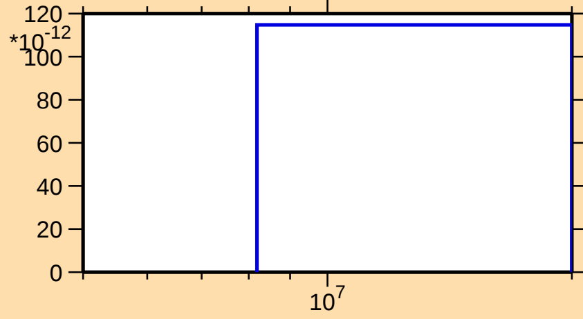
\sigma vs. E for ^{260}\text{Fm}(n,nd)
