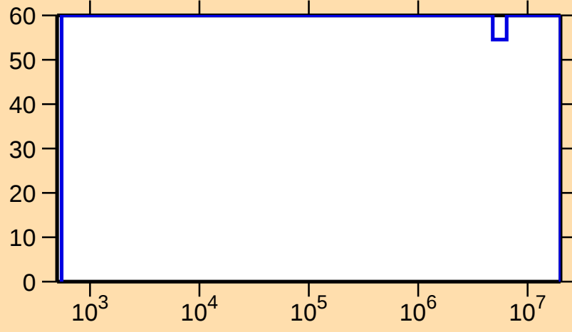
\Delta\sigma/\sigma vs. E for ^{260}\text{Fm}(n,\gamma)
