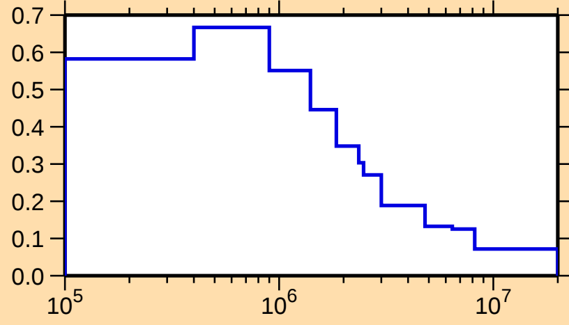
\sigma vs. E for ^{260}\text{Fm}(n,\text{inel.})
