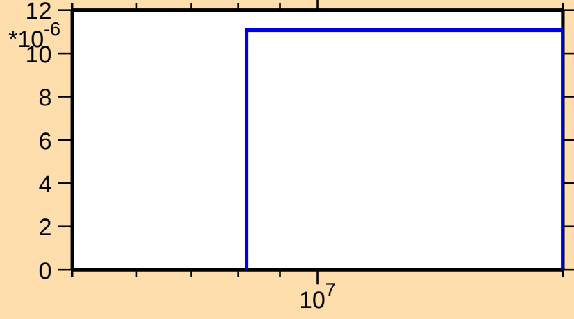
\sigma vs. E for ^{260}\text{Fm}(n,t)
