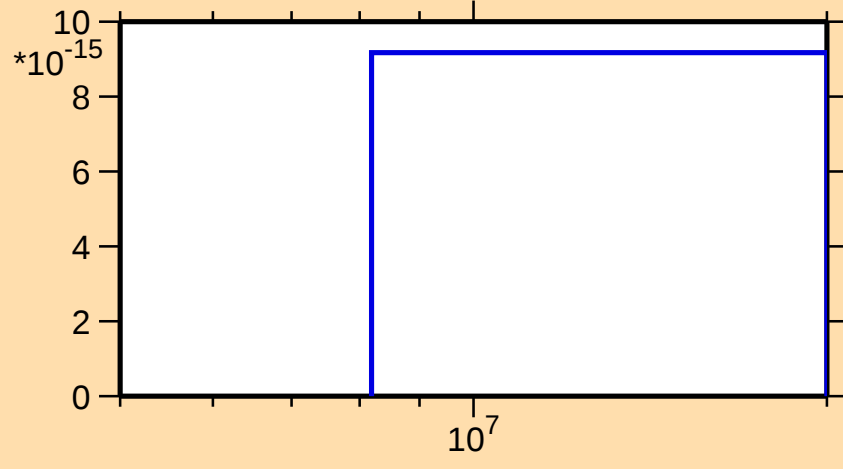
\sigma vs. E for ^{260}\text{Fm}(n,\text{He}3)
