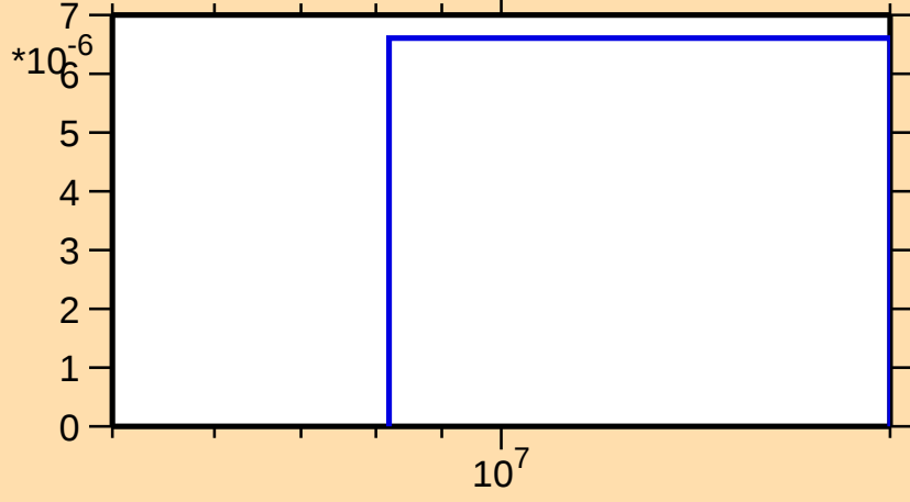
\sigma vs. E for ^{260}\text{Fm}(n,d)
