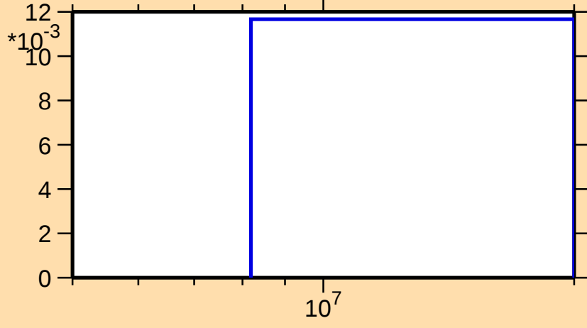
\sigma vs. E for ^{260}\text{Fm}(n,3n)
