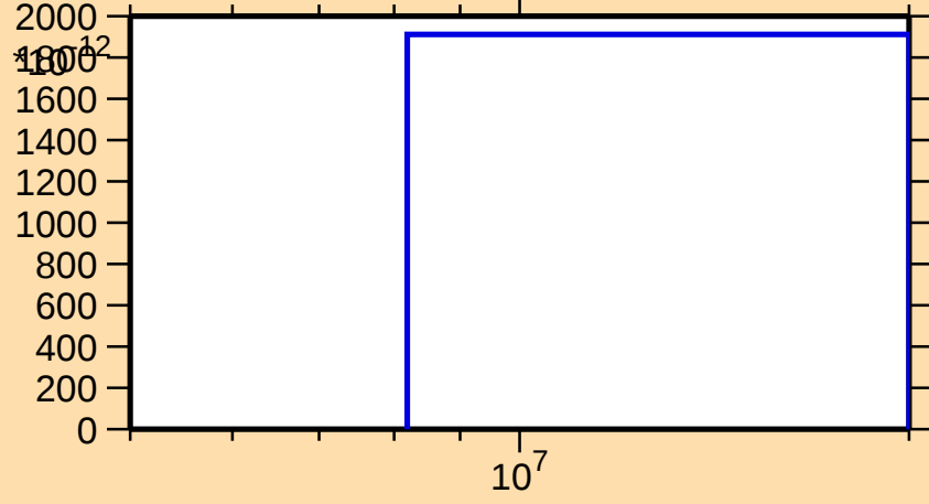
\sigma vs. E for ^{260}\text{Fm}(n,nt)
