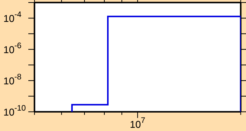
\sigma vs. E for ^{260}\text{Fm}(n,p)
