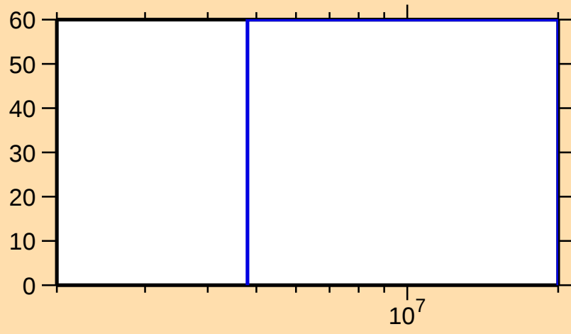
\Delta\sigma/\sigma vs. E for ^{260}\text{Fm}(n,2n)
