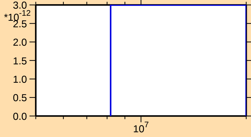
\sigma vs. E for ^{260}\text{Fm}(n,2np)
