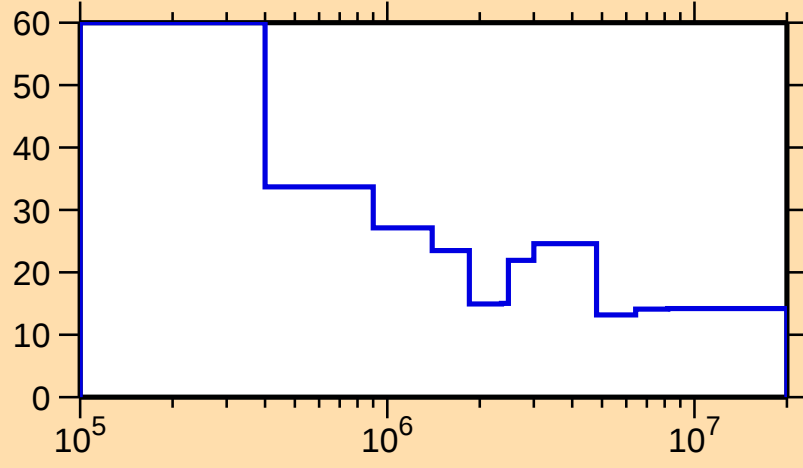
\Delta\sigma/\sigma vs. E for ^{260}\text{Fm}(n,f)
