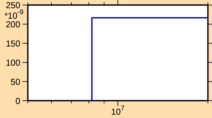
\sigma vs. E for ^{260}\text{Fm}(n,np)
