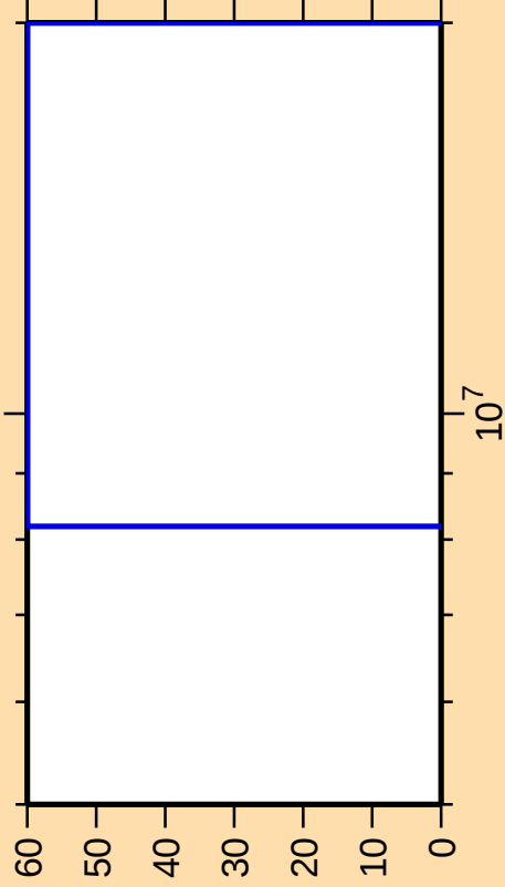
\Delta\sigma/\sigma vs. E for ^{260}\text{Fm}(n,nt)
