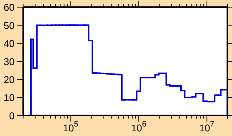
\Delta\sigma/\sigma vs. E for ^{145}\text{Gd}(n,\text{tot.})
