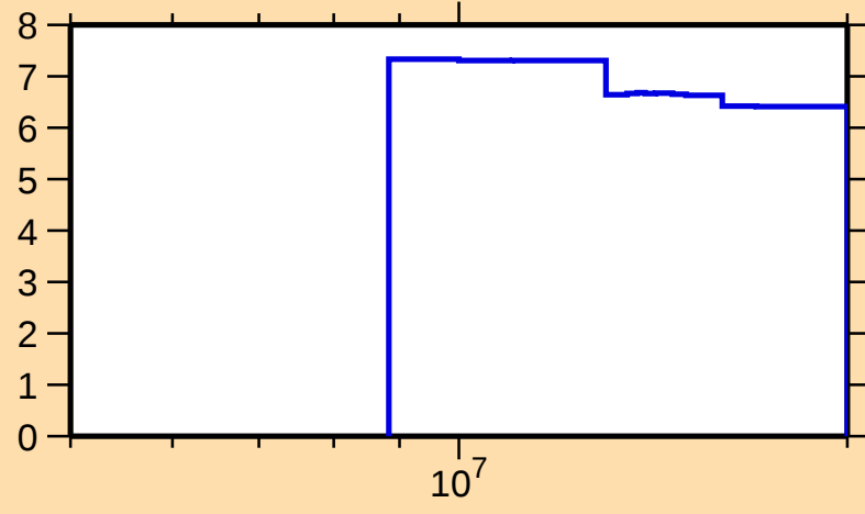
\Delta\sigma/\sigma vs. E for ^{145}\text{Gd}(n,\text{nonel.})
