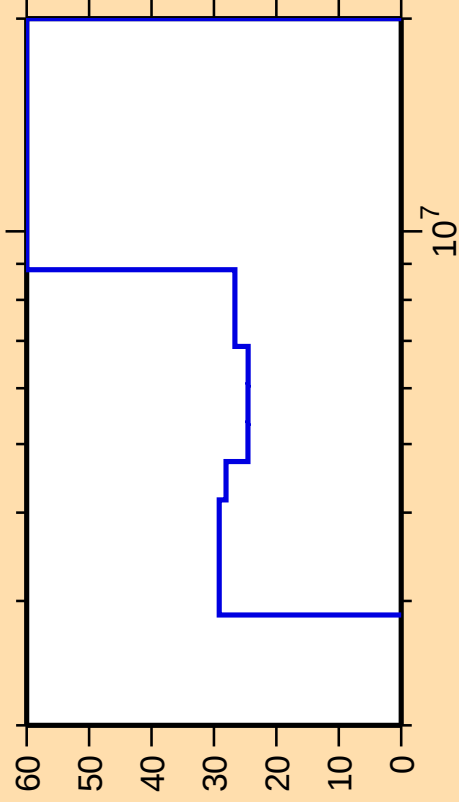
\Delta\sigma/\sigma vs. E for ^{145}\text{Gd}(n,\text{ncont.})
