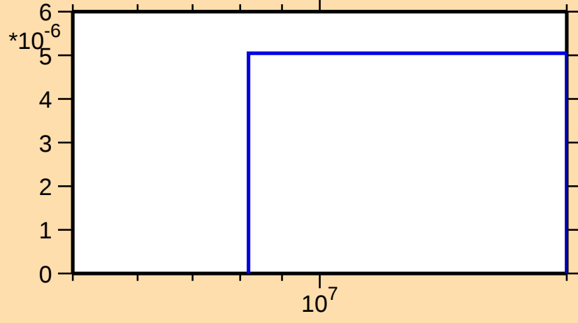
\sigma vs. E for ^{167}\text{Hf}(n,3n)
