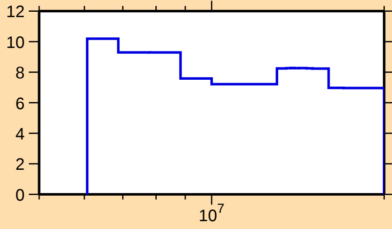
\Delta\sigma/\sigma vs. E for ^{197}\text{Hg}(n,\text{nonel.})
