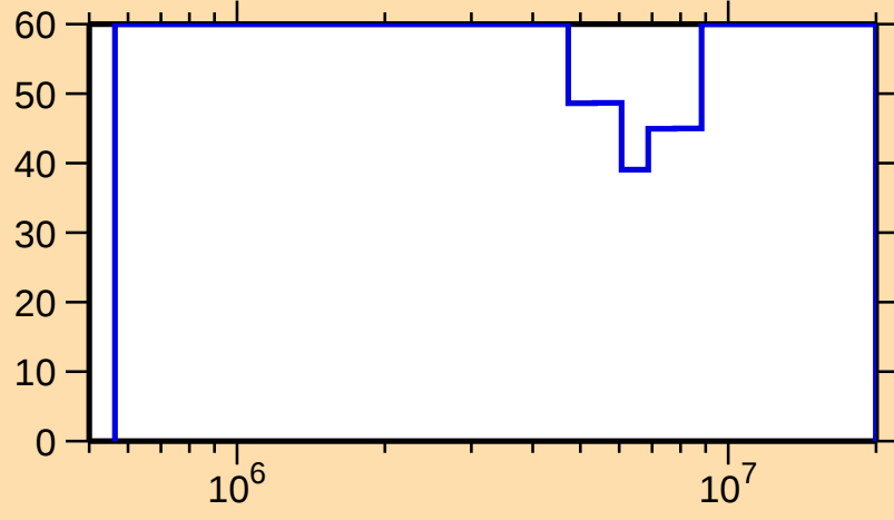
\Delta\sigma/\sigma vs. E for ^{197}\text{Hg}(n,\gamma)
