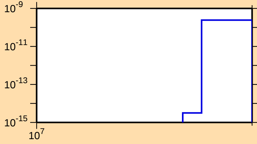
\sigma vs. E for ^{197}\text{Hg}(n,\text{nt})
