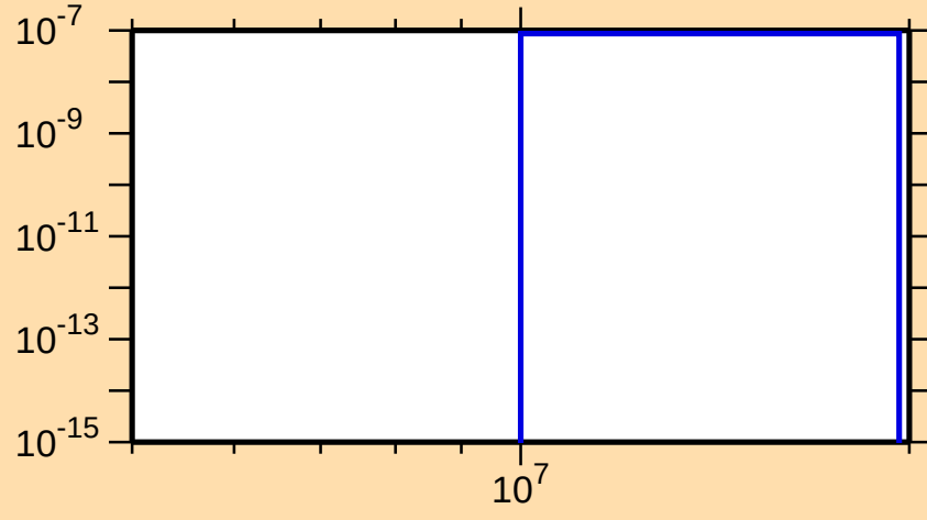
\sigma vs. E for ^{197}\text{Hg}(n,2n\alpha)
