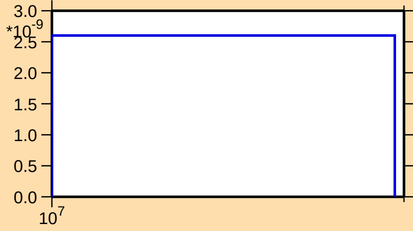
\sigma vs. E for ^{197}\text{Hg}(n,\text{nd})
