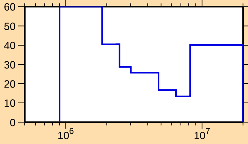
\Delta\sigma/\sigma vs. E for ^{197}\text{Hg}(n,n\text{cont.})
