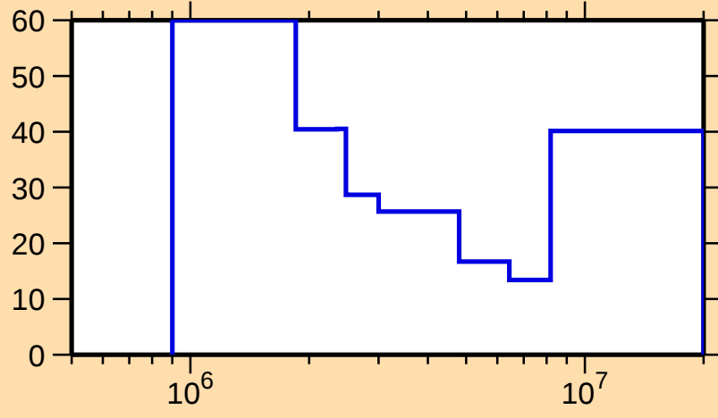
\Delta\sigma/\sigma vs. E for ^{197}\text{Hg}(n,n\text{cont.})
