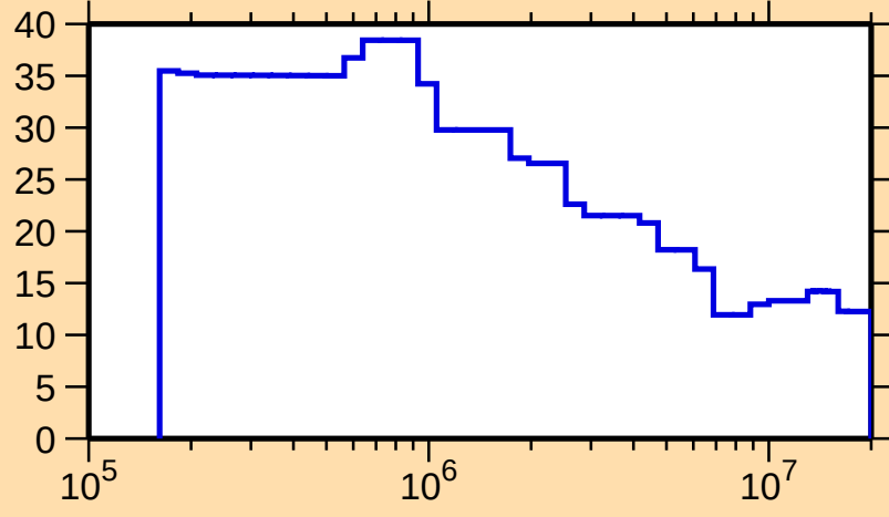
\Delta\sigma/\sigma vs. E for ^{146}\text{Ho}(n,\text{nonel.})
