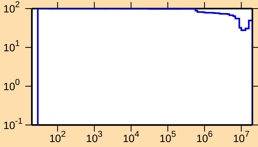
\Delta\sigma/\sigma vs. E for ^{146}\text{Ho}(n,\gamma)
