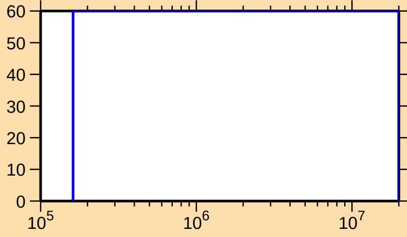
\Delta\sigma/\sigma vs. E for ^{146}\text{Ho}(n,n_1)
