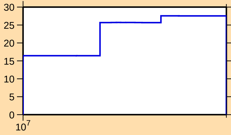
\Delta\sigma/\sigma vs. E for ^{146}\text{Ho}(n,\text{tot.})
