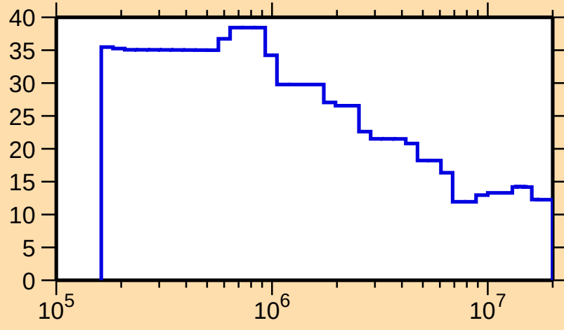
\Delta\sigma/\sigma vs. E for ^{146}\text{Ho}(n,\text{nonel.})
