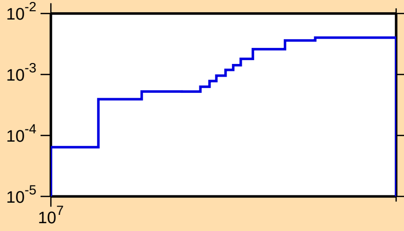
\sigma vs. E for ^{146}\text{Ho}(n,2n)
