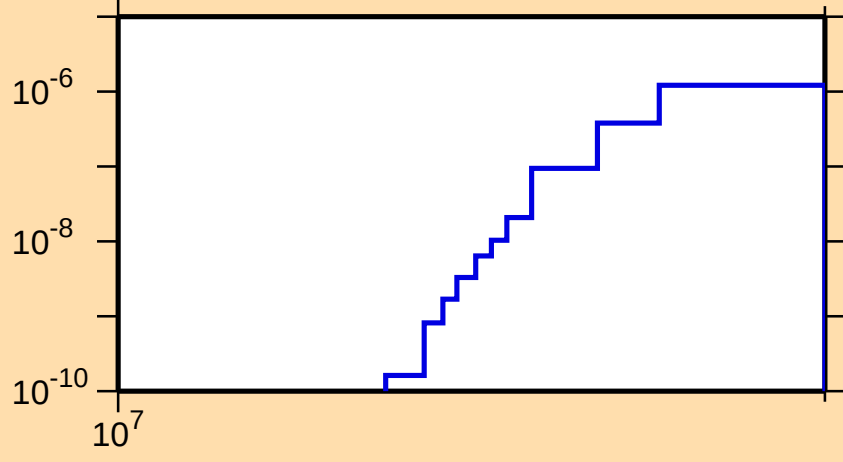
\sigma vs. E for ^{146}\text{Ho}(n,2n\alpha)
