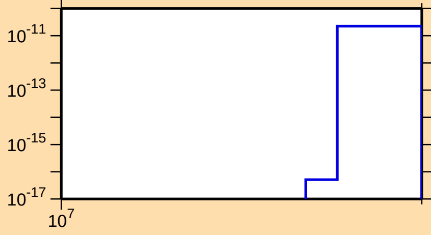
\sigma vs. E for ^{146}\text{Ho}(n,\text{nt})
