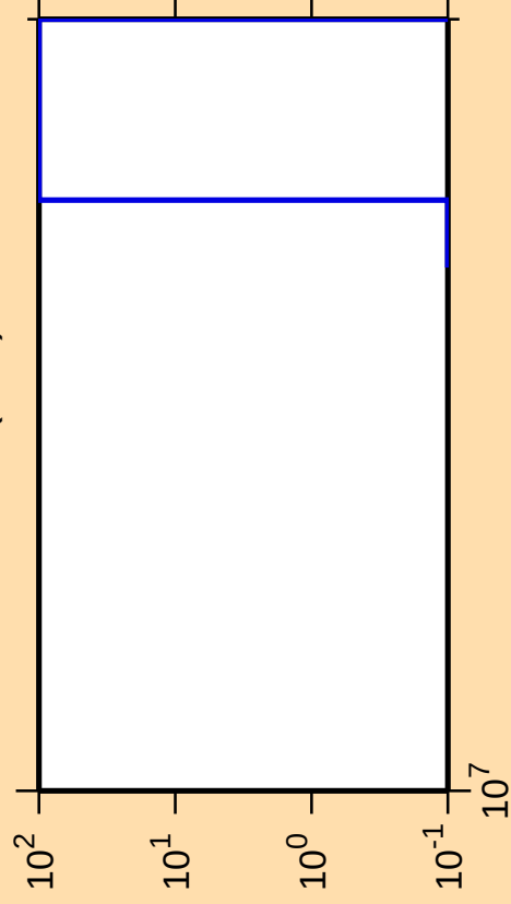
\Delta\sigma/\sigma vs. E for ^{146}\text{Ho}(n,\text{nt})
