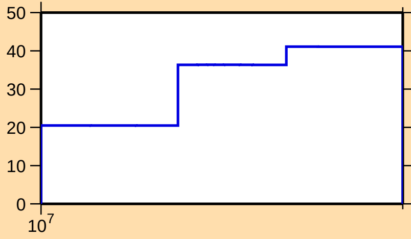
\Delta\sigma/\sigma vs. E for ^{146}\text{Ho}(n,\text{el.})
