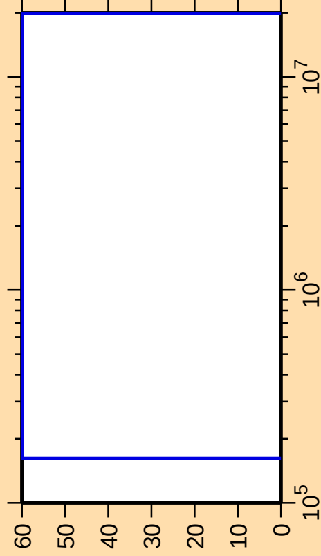
\Delta\sigma/\sigma vs. E for ^{146}\text{Ho}(n,\text{ncont.})
