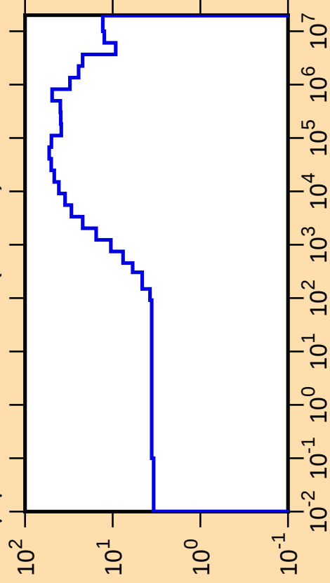
\Delta\mu/\mu vs. E for ^{146}\text{Ho}(\text{mt251})
