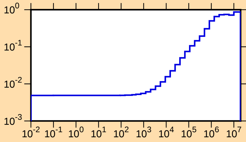
\mu vs. E for ^{146}\text{Ho}(\text{mt251})
