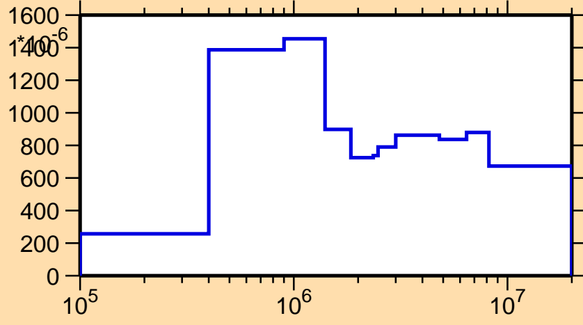
\sigma vs. E for ^{146}\text{Ho}(n,n_1)
