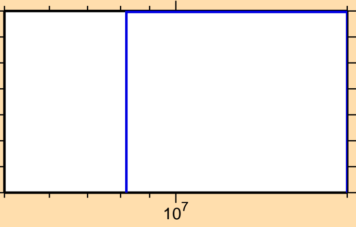
\sigma vs. E for ^{146}\text{Ho}(n,2np)
