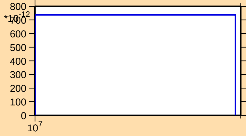
\sigma vs. E for ^{116}\text{In}(n,\text{nt})
