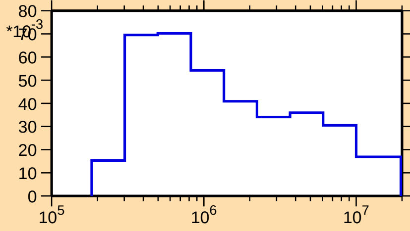
\sigma vs. E for ^{116}\text{In}(n,n_2)
